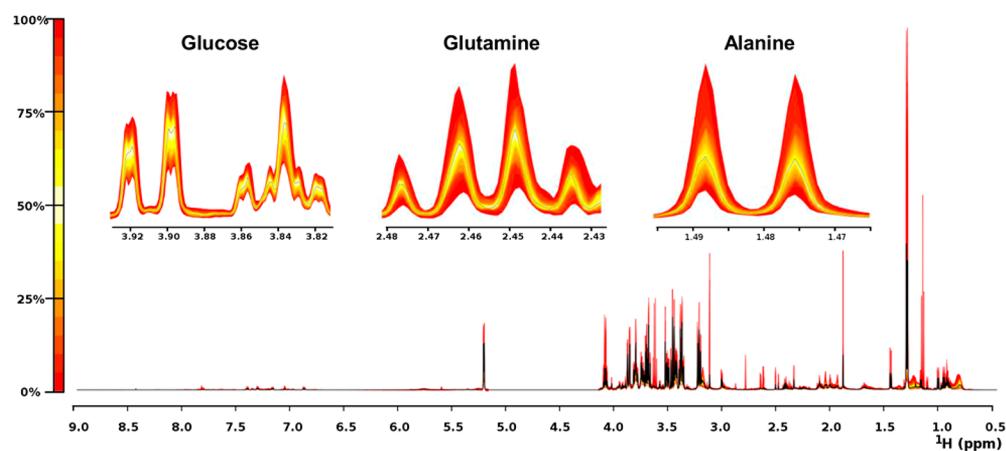
Figure 1. Quantile plots of OA/OC (Non-Septic), sepsis, and all spectra depicting the median spectral plot (black line) and variation from the median within each group (yellow to red scale) for the full spectral range (9.0–0.5 ppm) and more detailed regions depicting selected peaks from three differentially abundant metabolites, glucose, glutamine, and alanine. Variation within the full spectra can most clearly be seen at 0.8 ppm.
