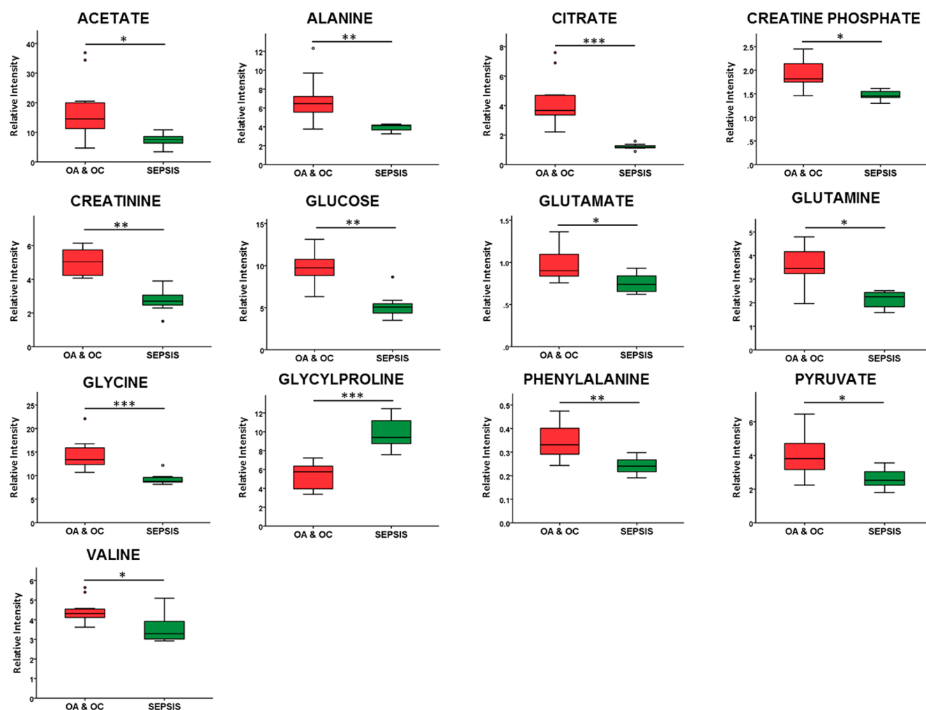
Figure 4. Boxplots of key metabolites, shown as relative intensities corresponding to the most representative peak for each metabolite. t test: * = p < 0.05 , ** = p < 0.01 , and *** = p < 0.001 .
