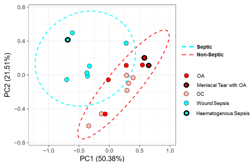
Figure 2. Principal component analysis (PCA) scores plot of septic (blue) and nonseptic (red) SF samples. Samples with meniscal tear or hematogenous sepsis subdiagnoses for OA and sepsis, respectively, are highlighted in each group with a thick black outline, OC are distinguished from OA by highlight shade.
