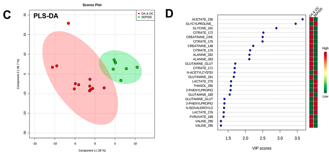
Figure 3. (a) PLS-DA plots of OA/OC versus sepsis using only metabolite annotated buckets: first two components shown out of a total of two components used to fit the model ( R^2 = 0.85 , Q^2 = 0.72 ). (b) VIP scores for the 25 most influential buckets of PLS-DA. (c) PLS-DA plots of OA/OCD versus sepsis using only metabolite annotated/identified buckets with all glucose buckets excluded: first two components shown. It should be noted that only one component was used to fit the model ( R^2 = 0.70 , Q^2 = 0.45 ). (d) VIP scores for the 25 most influential buckets of glucose-excluded PLS-DA.
