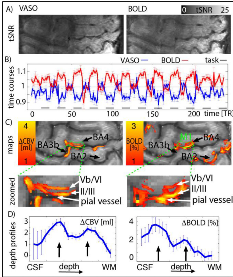
Fig. 3. Measures of functional stability and sensitivity from one representative participant. Panel A) depicts tSNR for VASO and BOLD contrast. Panel B) depicts the time course of a GM ROI in M1 (BA4) (same for VASO and BOLD, green in panel C). It can be seen that the signal change between tapping and resting periods is larger than the noise between consecutive time points. Panel C) depicts layer-dependent activity maps for VASO and BOLD. It can be seen that GE-BOLD signal is dominated by activity from superficial layers. In VASO, however, a double stripe pattern can be seen in the index-finger region of M1. Panel D) presents the signal change as a function of cortical depth. The profile shows a double peak (black arrows). For BOLD, the double-peak feature is overlaid with a gradient of decreasing signal change towards deeper layers. (one-column, 4'' width)
