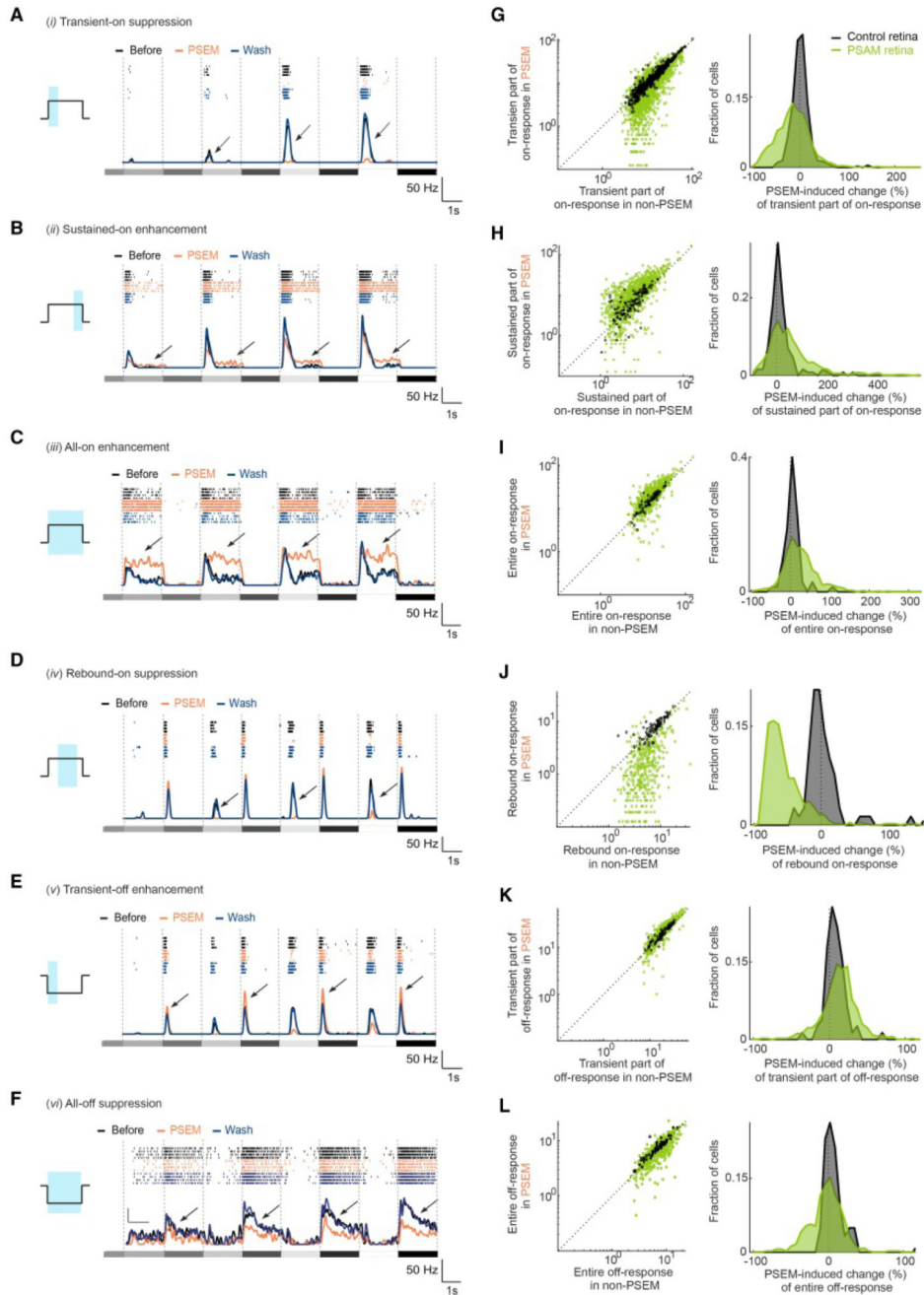
Figure 3. Horizontal cells shape the response dynamics of ganglion cells.
