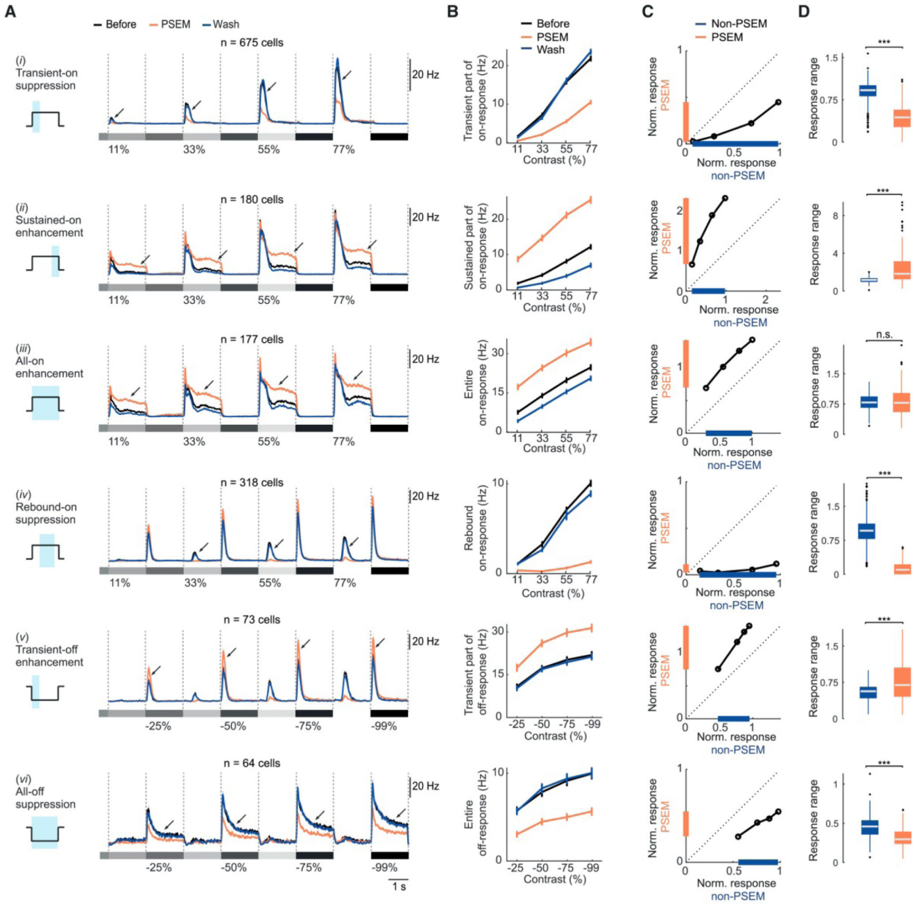
Figure 4. Horizontal cells influence the response range of ganglion cells.
