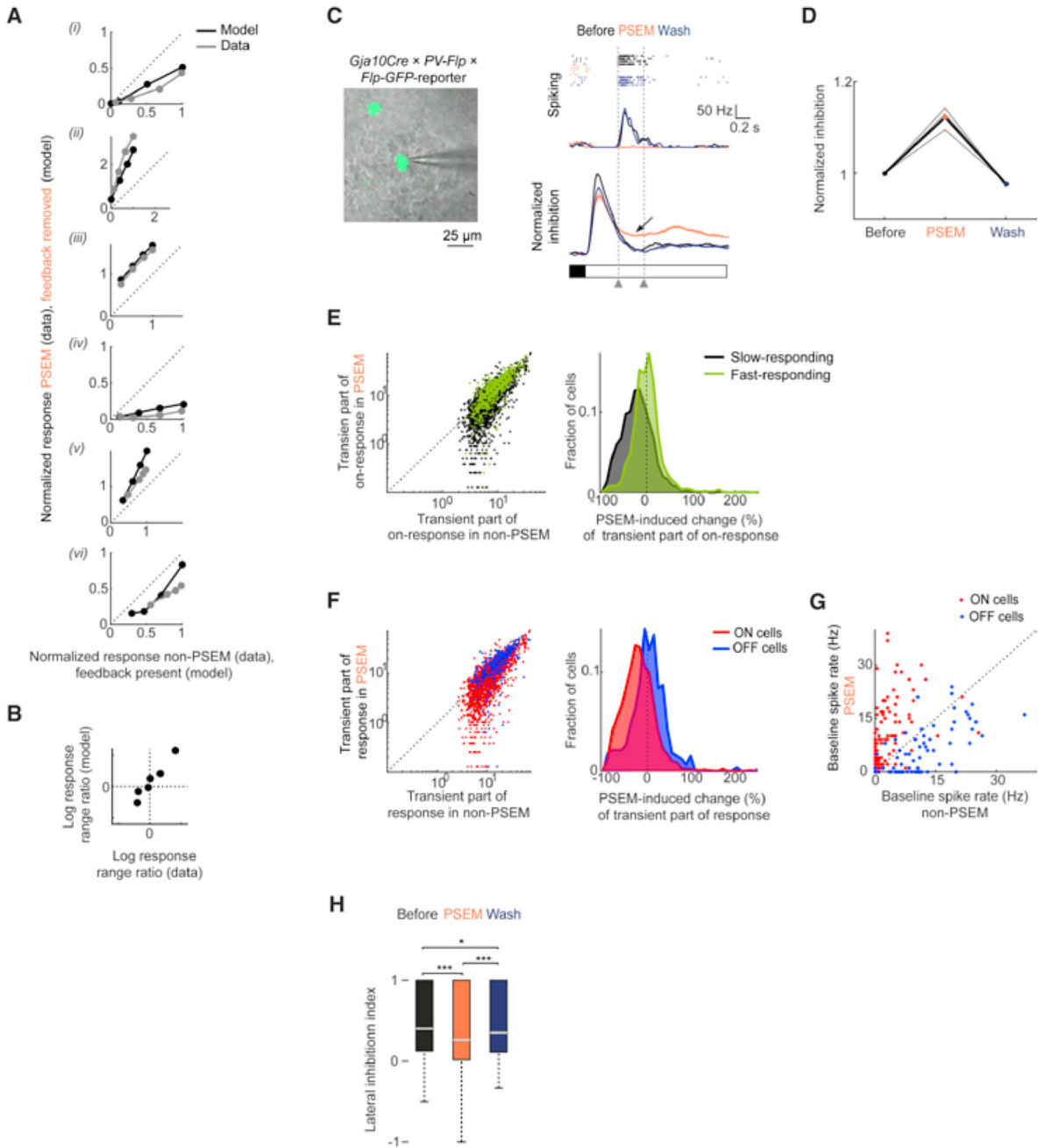
Figure 8. Experimental validation of model predictions.
