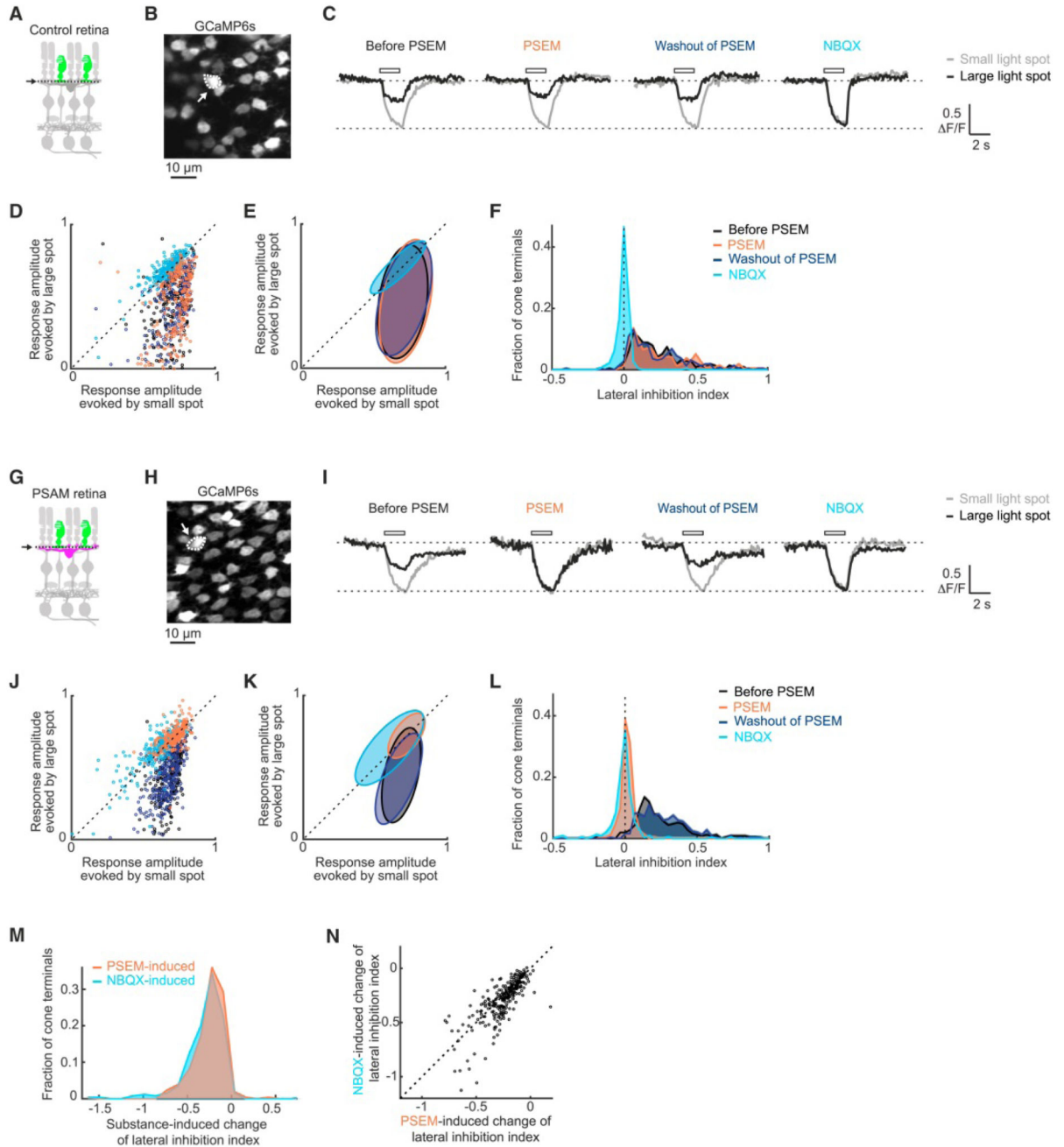
Figure 2. Reversible perturbation of horizontal cells.
