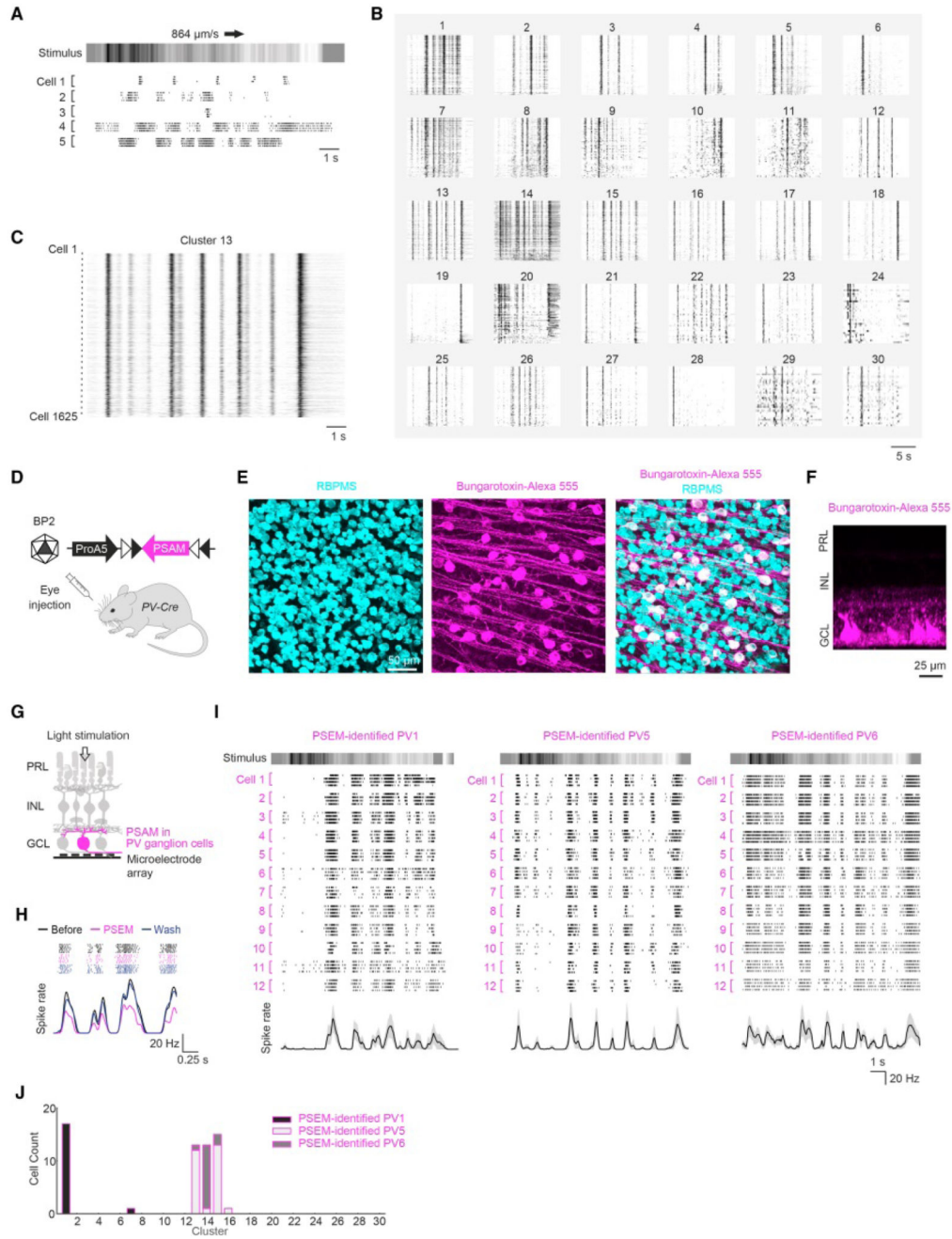
Figure 5. Cell-type identification on microelectrode arrays.
