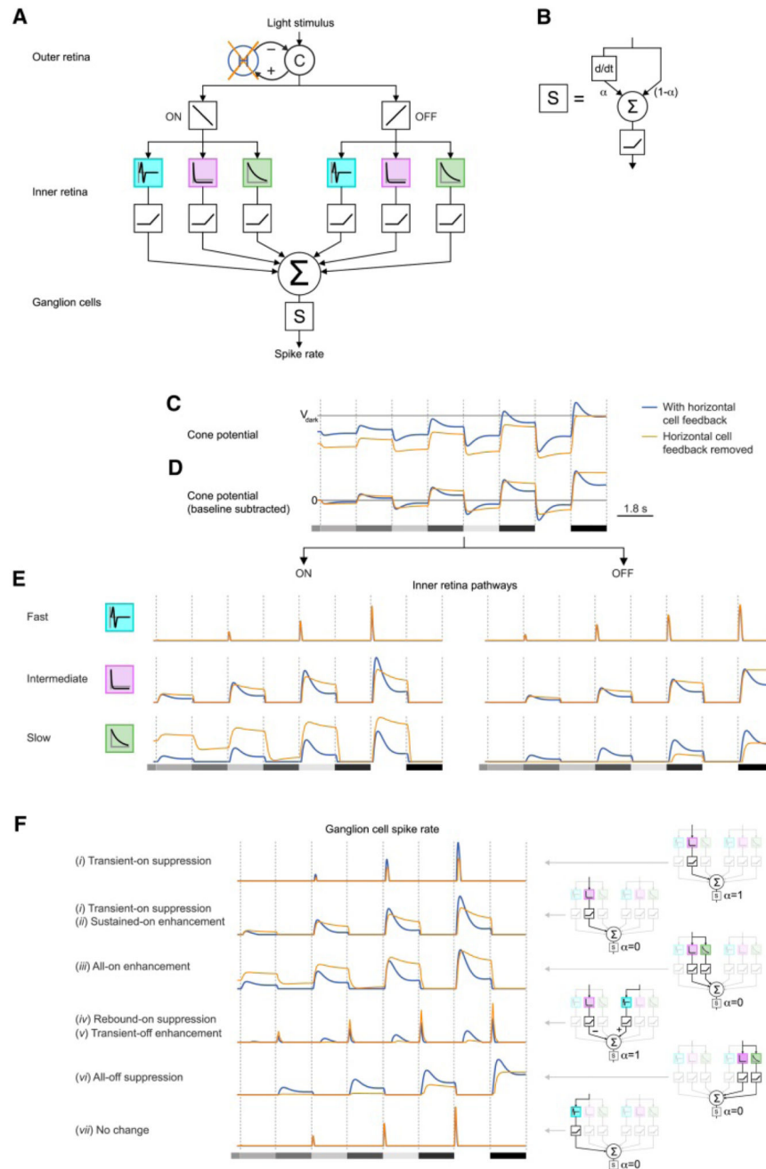
Figure 7. Computational model of the retinal circuitry explains all perturbation-induced effects. (A) Schematic of retinal circuit model. From top to bottom: cone (C)-horizontal cell (H) negative feedback circuit, subsequent split into ‘ON’ (left) and ‘OFF’ pathways (right), followed by filtering operations (colored boxes) and threshold non-linearities (black boxes) of inner retina pathways. Removal of horizontal cell feedback: orange cross. For each model ganglion cell, the inner retina pathways were linearly combined ( \Sigma ) and converted to a spike rate by function ‘S’. (B) Function S was the thresholded weighted average ( \Sigma , weighted by parameter \alpha ) of a ganglion cell’s previously combined inputs (right) and the temporal
