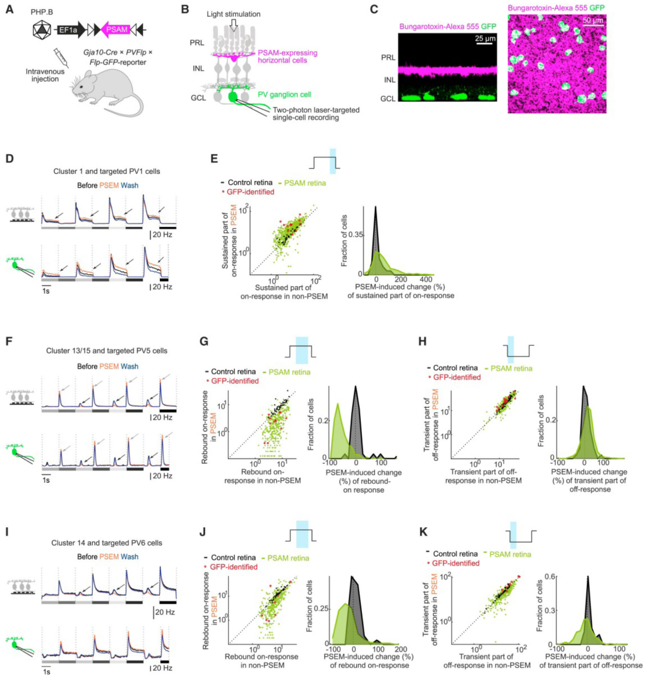
Figure 6. Horizontal cells differentially affect individual ganglion cell types.
