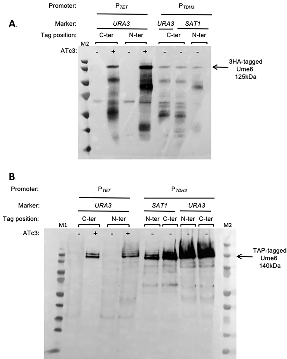
Figure 5. Detection of 3xHA- or TAP-tagged Ume6 protein by western blot. Production of 3xHA-tagged (A) and TAP-tagged (B) Ume6 proteins. Candida albicans strains harboring the P_{TET} and P_{TDH3} constructions were grown in YPD \pm ATc3 for 2 and 4 h, respectively. Whole cell extracts were separated by SDS-PAGE and probed with a peroxidase-coupled antibody, allowing the detection of the 3xHA-tagged and TAP-tagged Ume6 protein. The tagged Ume6 proteins are indicated by an arrow along with their deduced sizes. M1: PageRuler Prestained Protein Ladder (Thermo Scientific) and M2: Precision Plus Protein™ Dual Color Standards (Bio-Rad).
