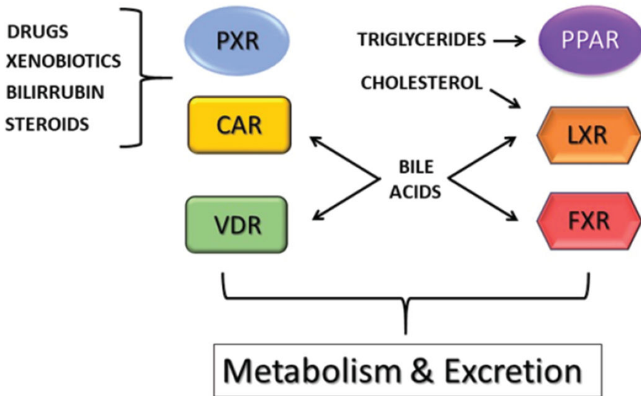
Figure 3: Endogenous and xenobiotic lipophilic ligands. Various xenobiotics and endogenous lipids are able to activate several nuclear receptors, which in turn control have the physiological role of controlling the intrahepatic and extrahepatic levels of these compounds. Thus, these receptors regulate the metabolism and excretion of these compounds. Note that a relatively high redundancy exists for several substance classes to bind to multiple receptors.
