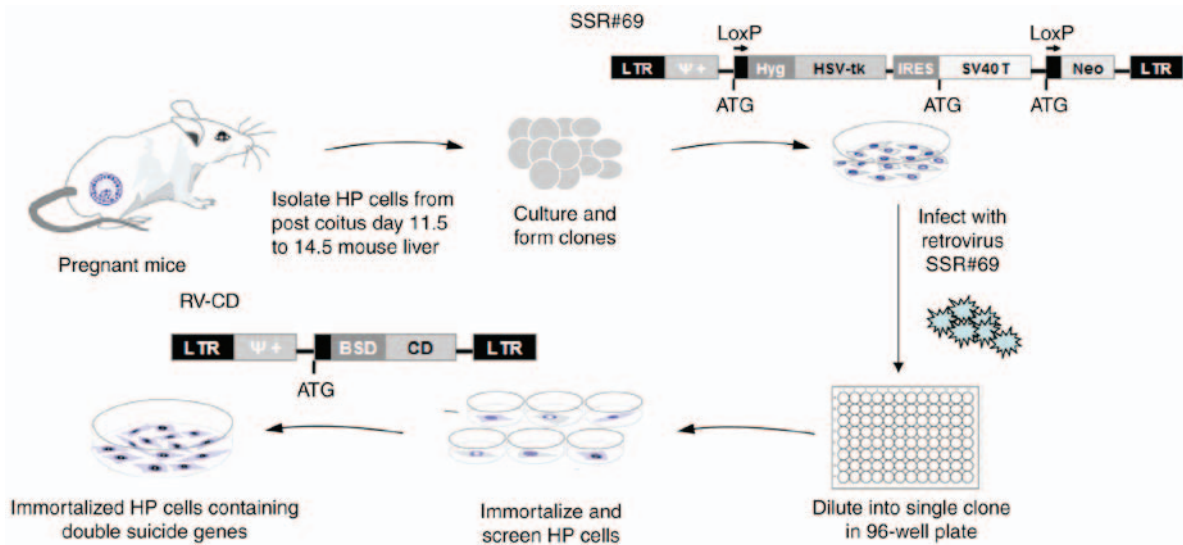
Figure 1. Flow diagram of the experimental procedure to produce the reversibly immortalized HP cells containing double suicide genes. HP, hepatic progenitor; LTR, long terminal repeat; Hyg, hygromycin; SV40T, simian virus 40 T-antigen; HSV-tk, herpes simplex virus thymidine kinase; BSD, blasticidin S; CD, cytosine deaminase; IRES, internal ribosome entry site; Neo, neomycin; RV-CD, retrovirus containing CD gene; SSR#69, retroviral vector expressing SV40T and Hyg-resistance genes flanked by paired LoxP recombination targets (12).
