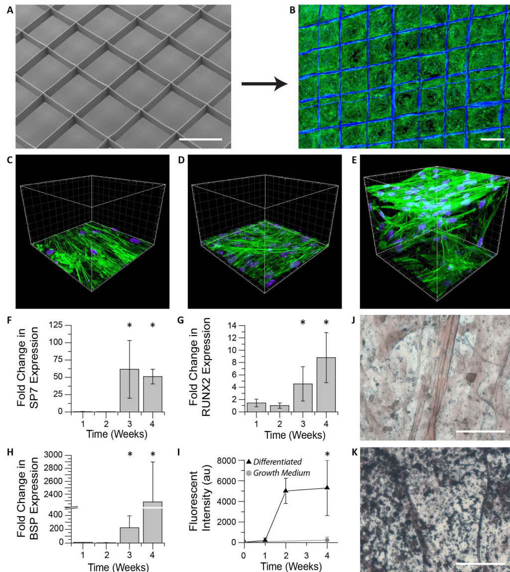
Figure 3. In vitro hMSC culture on 3D jet writing scaffolds produces 3D microtissues.
