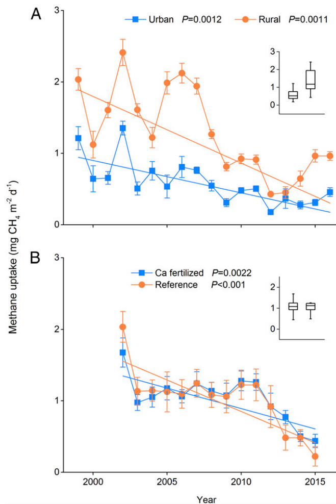
Fig. 1. Annual \text{CH}_4 uptake. (A) \text{CH}_4 uptake ( \pm SE, n = 8 –16) in urban and rural forests in Baltimore, Maryland, from 1999 to 2016 (annual means calculated for a “water year” from October to September). (B) \text{CH}_4 uptake ( \pm SE, n = 12 ) in calcium (Ca) fertilized and reference forests at Hubbard Brook, New Hampshire, from 2002 to 2015. Differences between forest types are significant in Baltimore (all P < 0.05 except in 2000 and 2013) but not significant (all P > 0.05 ) at Hubbard Brook for each year. The Insets represent average \text{CH}_4 uptake during the study period in urban ( Left ) versus rural ( Right , n = 18 , P < 0.001 ) or Ca-fertilized ( Left ) versus reference ( Right , n = 14 , P = 0.87 ) forests. The boxes show median and 5th and 95th percentiles. All trends with time are statistically significant ( P < 0.01 ) ( SI Appendix , Table S4).
