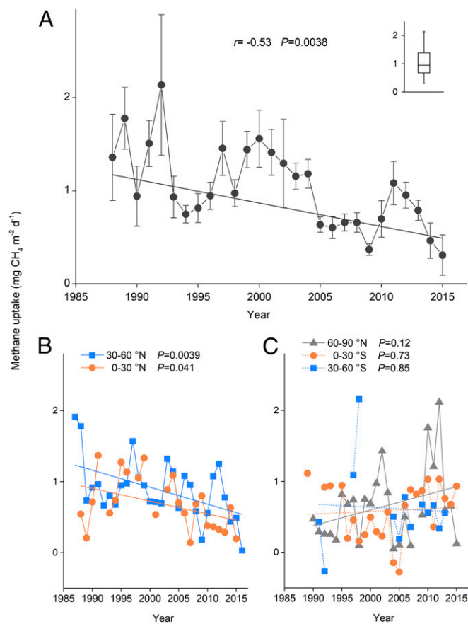
Fig. 2. Methane uptake in forest soils retrieved from published studies. (A) Global annual \text{CH}_4 uptake in forest soils from 1988 to 2015. The Inset represents average \text{CH}_4 uptake for the full period from 1988 to 2015. The boxes show median and 5th and 95th percentiles. Error bars denote SEs. (B) Annual \text{CH}_4 uptake in forest soils from 0 to 30^\circ \text{N} and 30 – 60^\circ \text{N} latitude. (C) Annual \text{CH}_4 uptake in forest soils from 60 to 90^\circ \text{N} , 0 – 30^\circ \text{S} and 30 – 60^\circ \text{S} latitude. All trends with time are statistically significant in A and B ( P < 0.05 ) ( SI Appendix , Table S4) but are not significant in C. The data in A were actually measured annual \text{CH}_4 uptake and those in B and C include both actually measured and estimated annual \text{CH}_4 uptake ( SI Appendix , Supplementary Methods ). The data collected in Baltimore and Hubbard Brook were excluded from this literature analysis.
