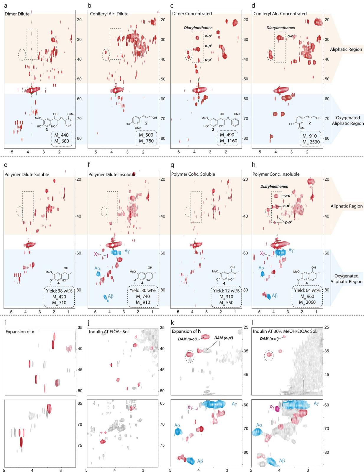
Fig. 5 ^1\text{H} - ^{13}\text{C} HSQC spectra of the reaction products obtained from kraft treatment of (a–d) guaiacylglycerol- \beta -guaiacyl ether (3) and (e–h) a \beta -O-4 phenolic model polymer (4). (i–l) Comparisons of selected regions of the HSQC NMR spectra from the reactions of the model compounds and of kraft lignin fractions. The structure in each panel shows the starting materials used to generate each synthetic kraft lignin. All M_n and M_w values are rounded to the nearest 10. Starting polymer M_n = 1490 , M_w = 2780 . The red colored contours in (i–l) indicate similarities between spectra. Blue and pink contours represent \beta -O-4 linkages and cinnamyl alcohol groups, respectively. The cross peak at \delta_{\text{H}}/\delta_{\text{C}} = 4.4/36.3 ppm (highlighted by the dashed circle) appears to be particularly diagnostic for a coniferyl alcohol pathway.
