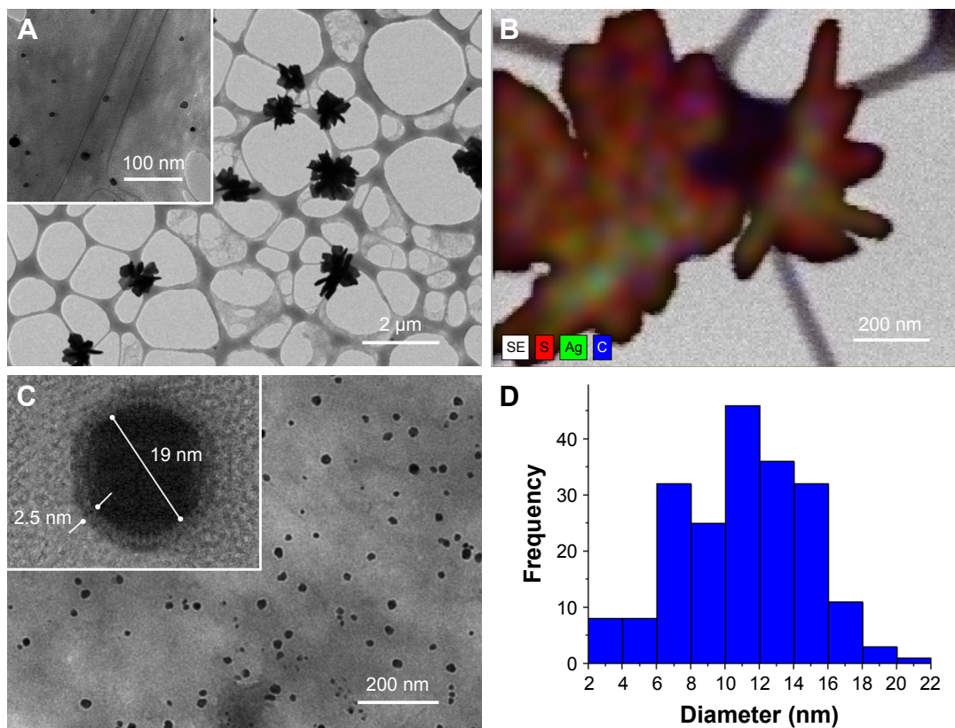
Figure 6 (HR-)TEM images of (A) SECS VS @Ag (DS SE 0.69) and (C) SECS BES @Ag (DS SE 1.05); (B) TEM/EDX image of SECS VS @Ag; (D) size distribution histogram of SECS BES @Ag (based on TEM images).
