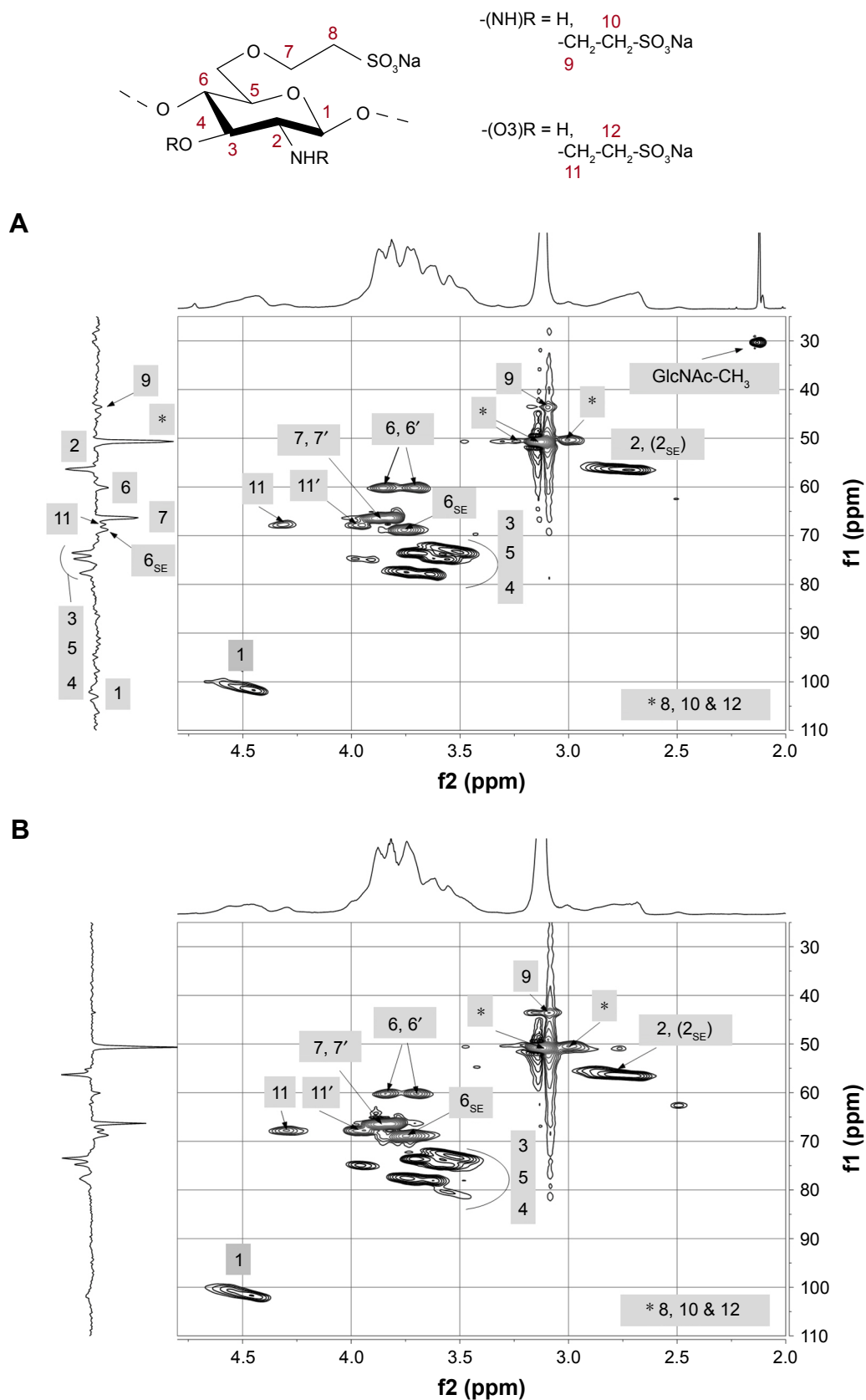
Figure 5 ^{13}\text{C} DEPT-135 edited HSQC NMR spectra of (A) \text{SECS}_{\text{VS}} ( \text{DS}_{\text{SE}} 0.69) and (B) \text{SECS}_{\text{BES}} ( \text{DS}_{\text{SE}} 1.05).
