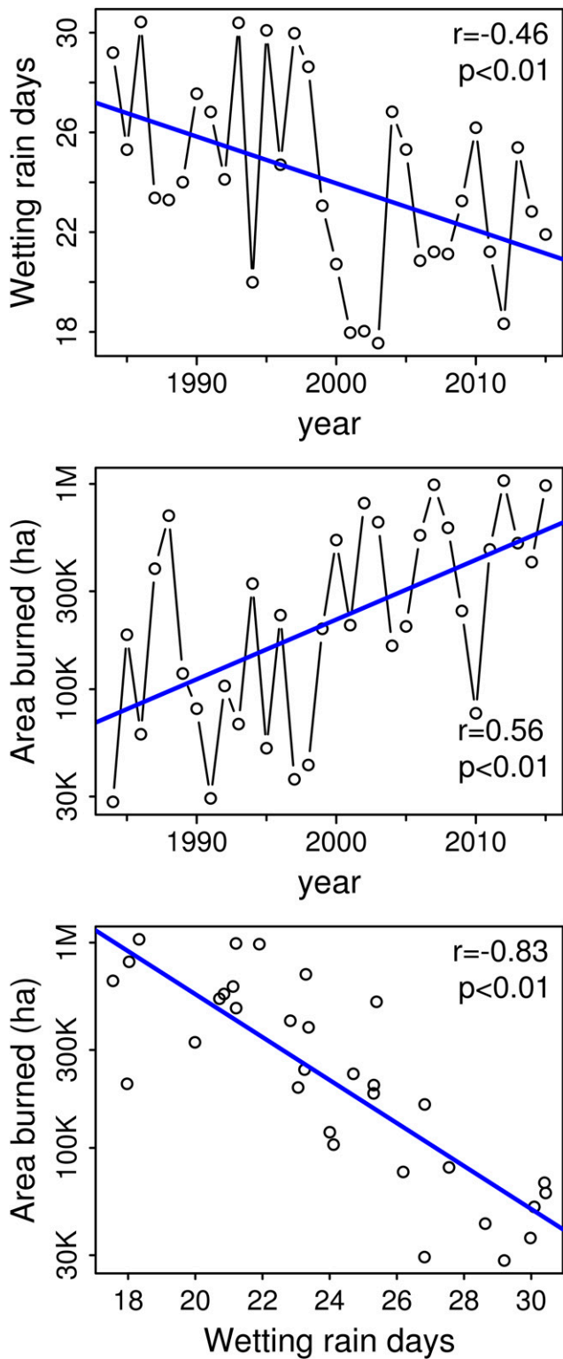
Fig. 4. Linear trends in WRD (Top), log-transformed wildfire area burned (Middle), and their correlation (Bottom) from 1984 to 2015 in forested areas of the western United States.
