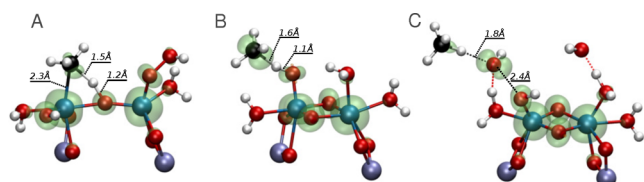
Figure 4. Transition states typical for (A) heterolytic dissociation, reaction 5 \rightarrow 9 ; (B) homolytic dissociation, reaction 26 \rightarrow 27 ; and (C) Fenton-type dissociation, reaction 2 \rightarrow 13 . The isosurface represents the spin density. Color coding: Al, purple; Fe, blue; O, red; C, black; H, white. The clusters shown here are part of a periodic model containing the unit cell of ZSM-5 zeolite, the Fe cluster, and the reactants.
