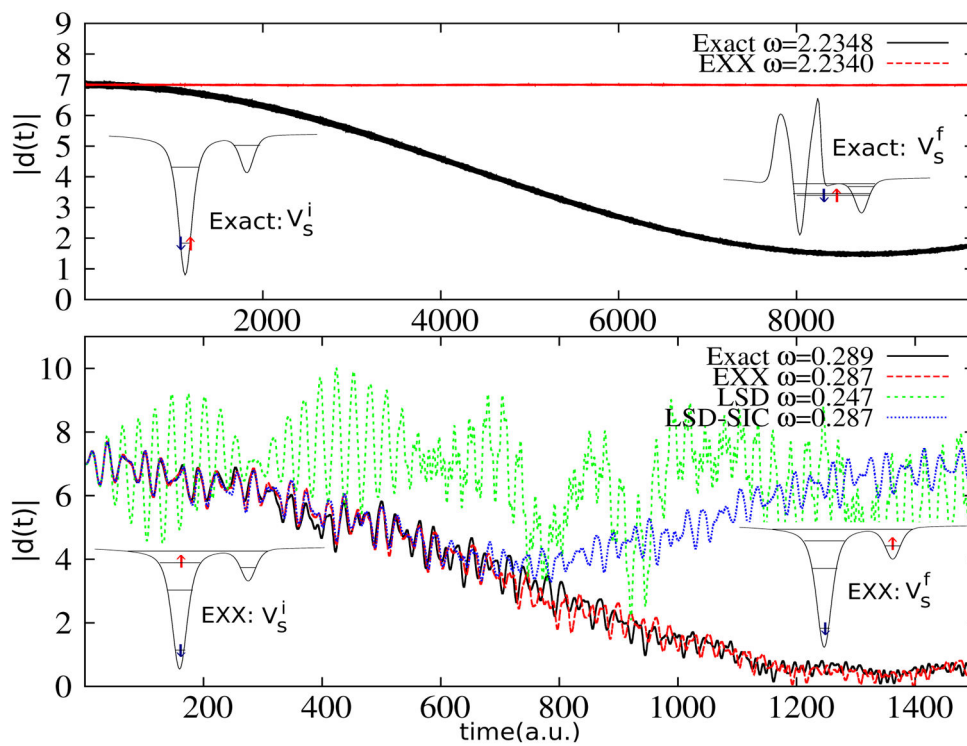
FIG. 1. Dipole moments calculated from the center of the double-well: exact (black), EXX (red), LSD (green) and SIC-LSD (blue), driven at resonant \omega^i for each. The initial and target-final KS potentials are shown as insets, exact in the top panel, and in EXX in the lower panel. Top panel: CT from the ground-state. Lower panel: CT from the “photo-excited” state.
