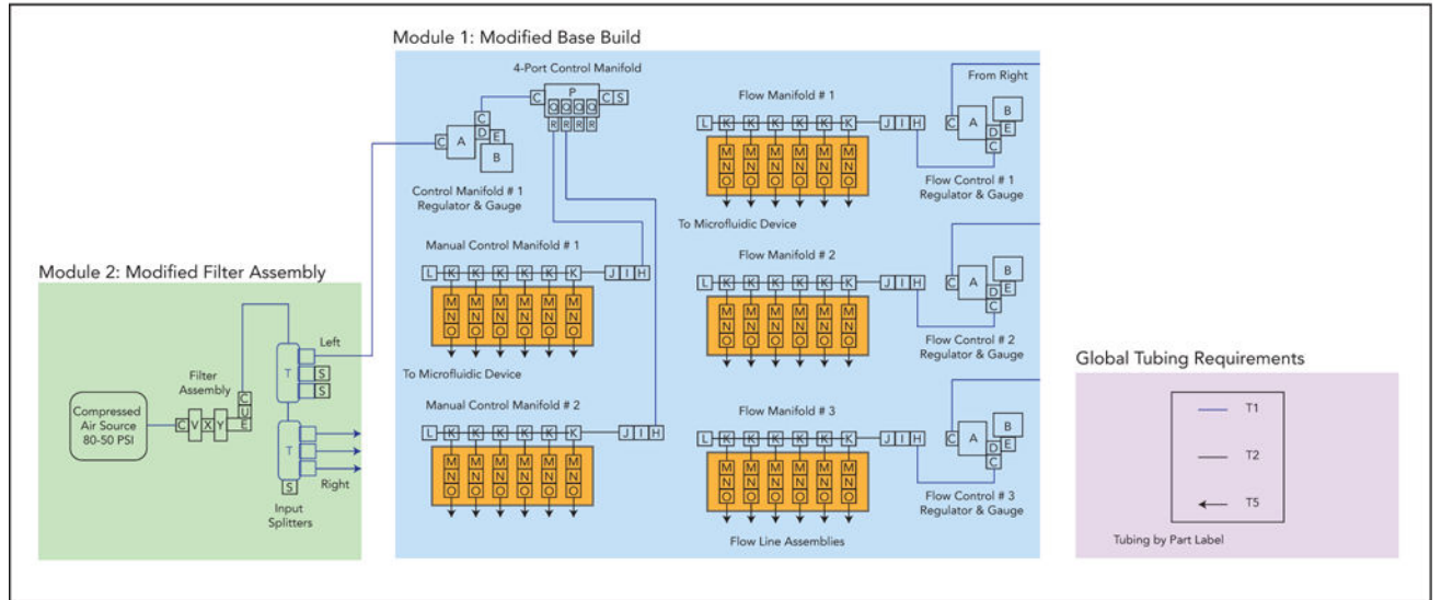
Figure 9. Build Option 3 schematic.
