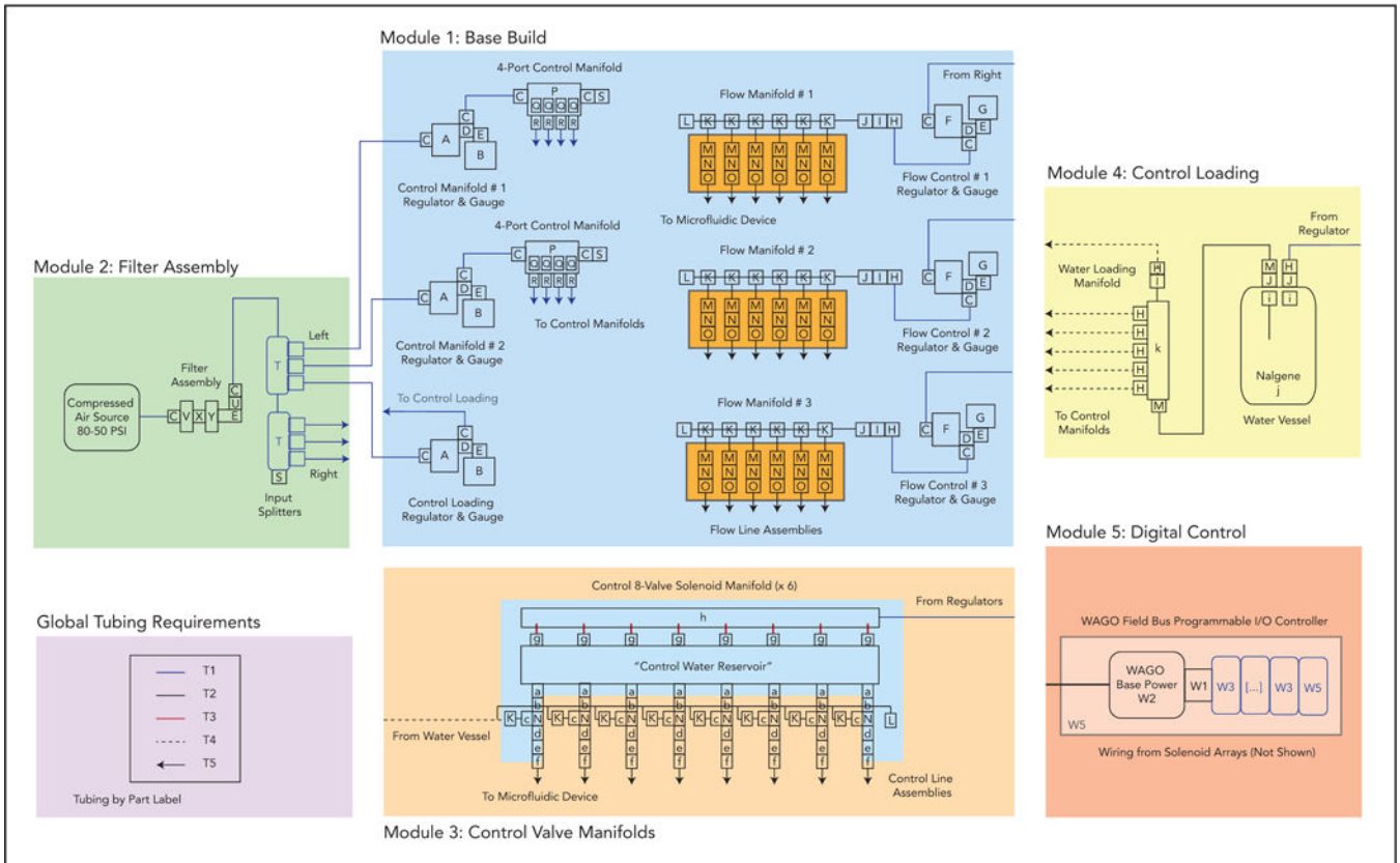
Figure 2. Overall setup schematic with parts designated by letter and number (as referenced to the Bill of Materials).
