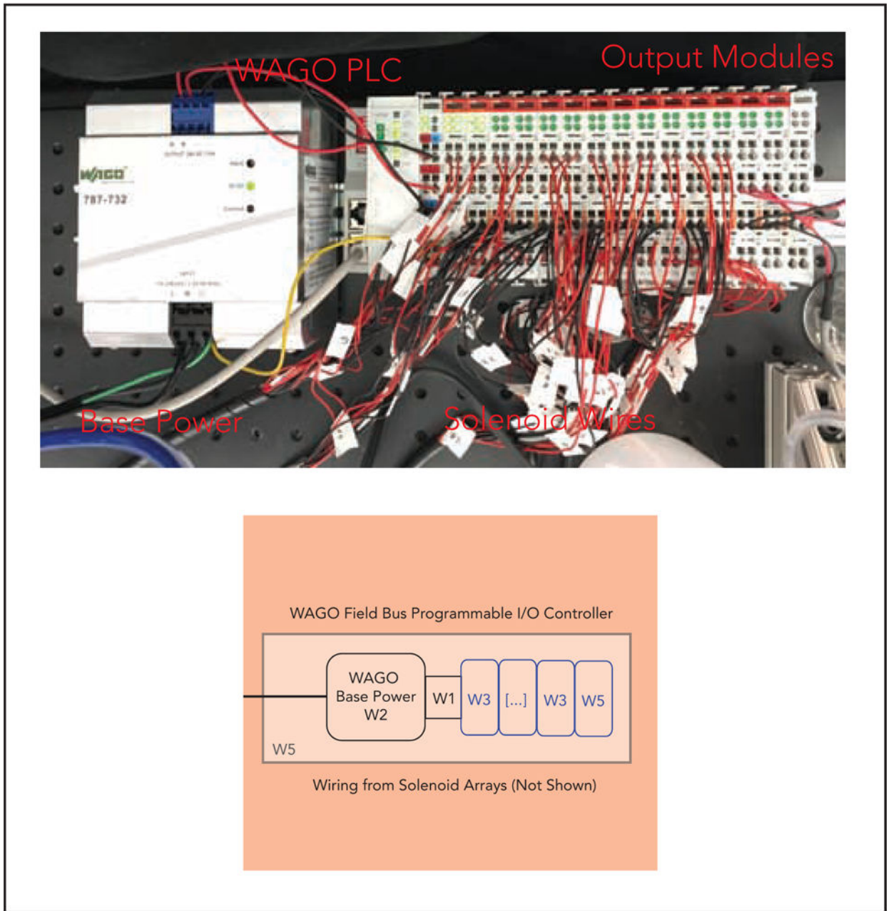
Figure 7. Module 5. (a) Module 5 schematic. (b) Finalized implementation of Module 5.
