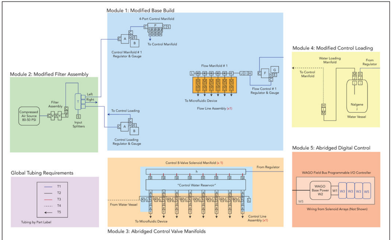
Figure 8. Build Option 2 schematic.
