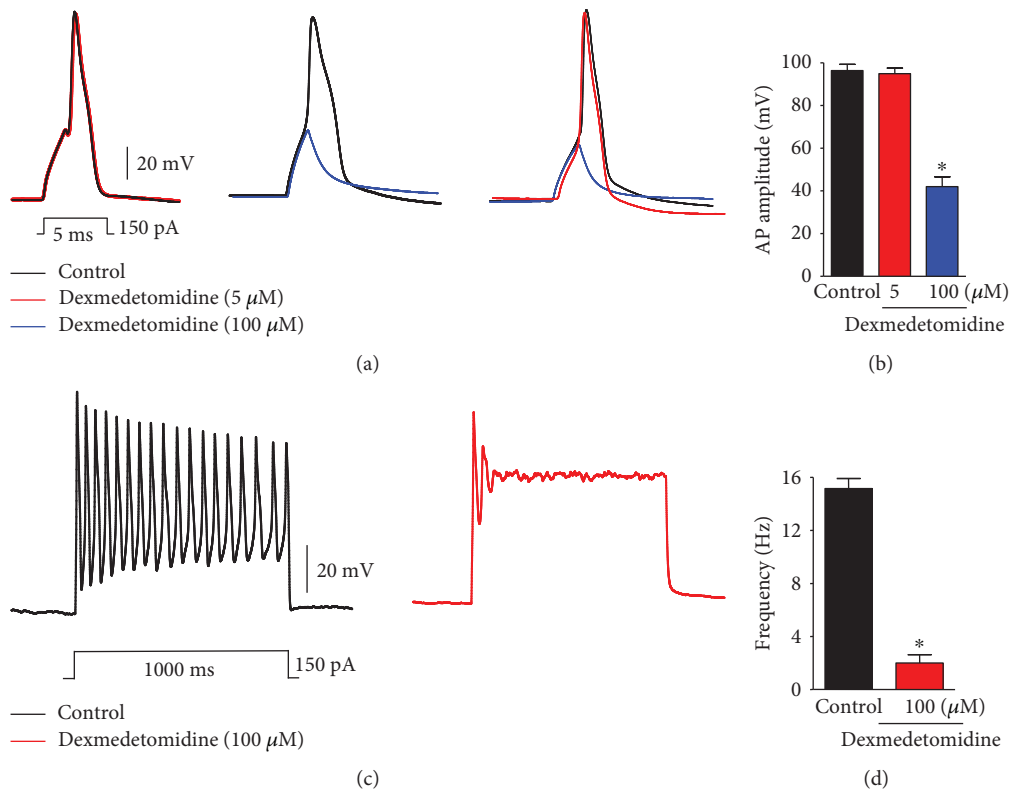
FIGURE 3: Effects of dexmedetomidine on action potentials (APs) in small-sized TG neurons. (a) Dexmedetomidine (100 \mu M) suppresses APs following current injection (5 ms, 150 pA) in small-sized TG neurons. Traces of single action potentials before (control) and after treatment with dexmedetomidine (5 and 100 \mu M). (b) Percent inhibition of AP amplitude by dexmedetomidine (5 and 100 \mu M). * p < 0.05 ; t -test versus control; n = 15 and 20 neurons per group, respectively. n.s.: no significance. (c) Dexmedetomidine inhibits the AP frequency after current injection (1 s, 150 pA) in small-sized TG neurons. Traces of action potentials before (control) and after treatment with dexmedetomidine (100 \mu M). (d) Dexmedetomidine (100 \mu M) markedly suppresses 90% of the AP frequency after current injection (150 pA) * p < 0.05 ; t -test versus control; n = 15 and 20 neurons per group, respectively.
