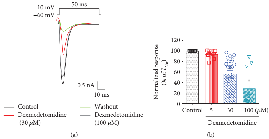
FIGURE 2: Effects of dexmedetomidine on voltage-gated sodium channel currents ( I_{Na} ) in small-sized TG neurons. (a) Dexmedetomidine suppresses I_{Na} in a concentration-dependent manner. Traces showing I_{Na} , the effects of dexmedetomidine (30, 100 \mu M), and the washout. (b) Percent inhibition of I_{Na} by dexmedetomidine (5 \mu M, n = 15/25 ; 30 \mu M, n = 20/32 ; 100 \mu M, n = 10/16 ). Results are presented as mean \pm SEM. * p < 0.05 ; t -test versus control; n = 10 –20 neurons per group.
