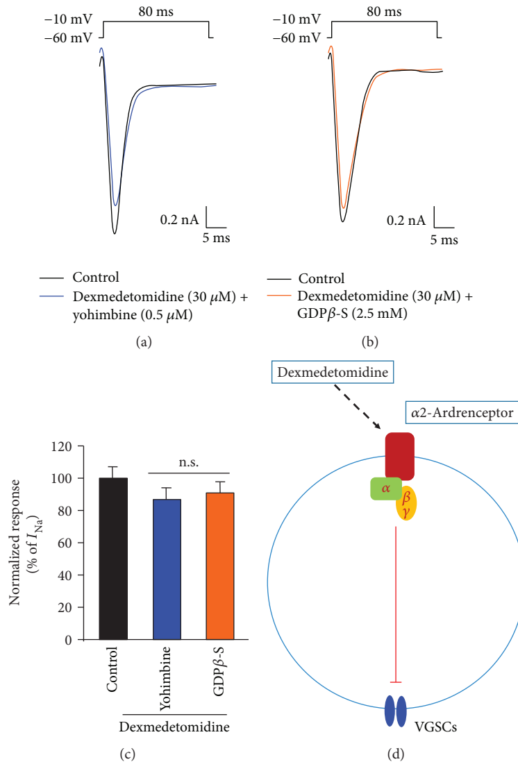
FIGURE 4: Effects of dexmedetomidine on I_{\text{Na}} via Gi/o protein-coupled \alpha_2 -adrenoceptors in small-sized TG neurons. (a) Treatment with yohimbine (0.5 \mu\text{M} , 2 min) suppresses the inhibitory effects of dexmedetomidine on I_{\text{Na}} in small-sized TG neurons ( n = 15 ). (b) Intracellular perfusion with GDP \beta -S (2.5 mM, 8 min) blocks inhibition of I_{\text{Na}} by dexmedetomidine ( n = 10 ). (c) Summary of inhibitory yohimbine and GDP \beta -S effects on the dexmedetomidine-mediated inhibition of I_{\text{Na}} . Results are presented as mean \pm SEM. n.s.: no significance. (d) Working hypothesis for the inhibition of I_{\text{Na}} by dexmedetomidine via Gi/o protein-coupled \alpha_2 -adrenoceptors in small-sized TG neurons. Sensory TG neurons do not only express neuronal VGSCs and Gi/o protein-coupled \alpha_2 -adrenoceptors. Stimulation of the \alpha_2 -adrenoceptor by dexmedetomidine suppresses the activity of VGSCs by inhibitory GPCR pathways in dissociated small-sized TG neurons.
