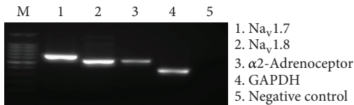
FIGURE 1: Expression of Na v 1.7, Na v 1.8, and the α2-adrenoceptor in TG neurons.
