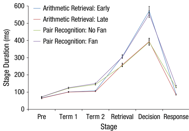
Fig. 4. Estimated duration of the six stages for the two conditions in each experiments. Error bars represent standard errors of the mean.
