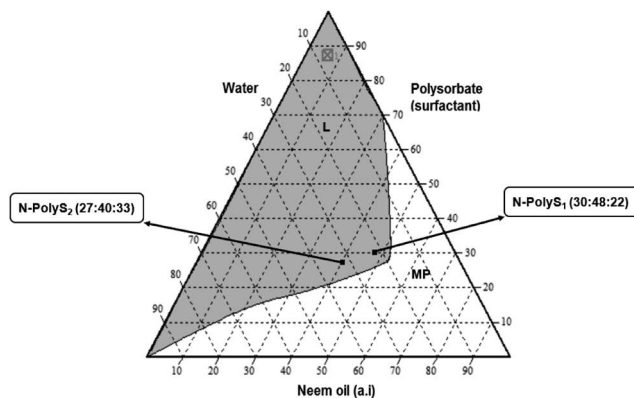
Fig. 2. Pseudoternary phase diagram of the polysorbate surfactant (Tween80)/neem oil/water) system, showing the selected nano-emulsion formulations with the ratios of N-PolyS 1 (30:48:22) and N-PolyS 2 (27:40:33). L=Isotropic. MP=Multiphase.
