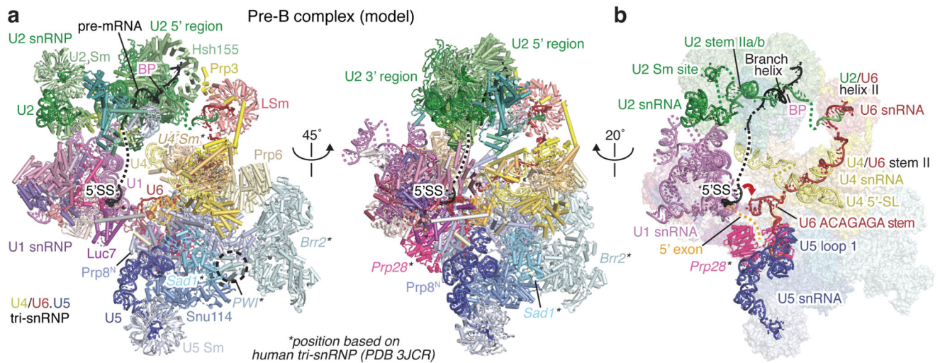
Figure 3. Spliceosome assembly and 5'SS transfer.
