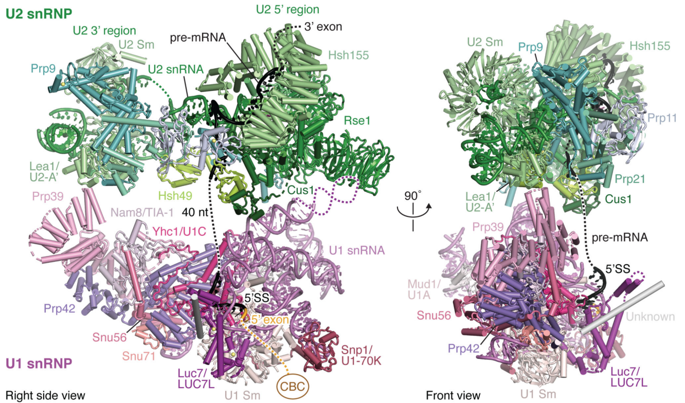
Figure 1. Prespliceosome A complex structure.
