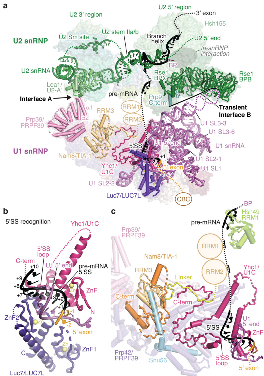
Figure 2. 5'SS recognition and implications for alternative splicing.
