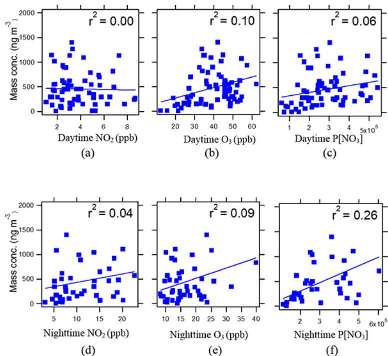
Figure 7. Correlation of IEPOX-derived SOA tracers with (a) daytime \text{NO}_2 , (b) daytime \text{O}_3 , (c) daytime \text{P}[\text{NO}_3] , (d) nighttime \text{NO}_2 , (e) nighttime \text{O}_3 , and (f) nighttime \text{P}[\text{NO}_3] . Nighttime \text{P}[\text{NO}_3] correlation suggests that \text{NO}_3 radical chemistry could explain some fraction of the IEPOX-derived SOA tracer concentrations. The contribution of nighttime \text{P}[\text{NO}_3] to IEPOX-derived SOA would be smaller than MAE/HMML-derived SOA due to the weaker correlation.
