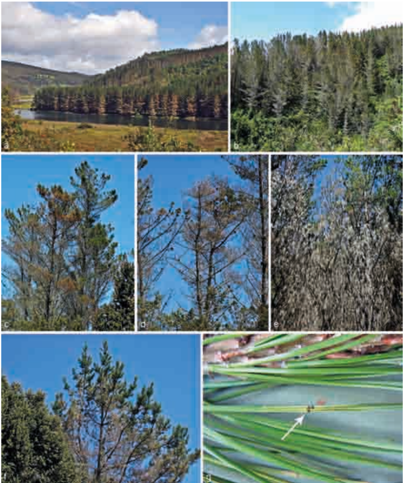
Fig. 13 Needle cast and defoliation caused by Phytophthora pinifolia on Pinus radiata in the Valdivian region of Chile. a. Mature plantation with extensive red-brown discoloration of infected foliage; b. mature plantation with largely defoliated crowns due to massive needle infections by P. pinifolia ; c. extensive defoliation of mature crowns resulting from the progressive browning and shedding of infected needles which started at the lowest branches and spared only the youngest needles; d. recently killed tree with severe defoliation; e. dying young tree in a dense stand with greyish discoloration of infected needles; f. upper crown typically showing transparency due to shedding of older infected needles, pale-green discolouration of freshly infected needles and uninfected, dark-green young needles; g. needle showing typical black bands (translucent areas; arrow) within the pale-green to greyish area of infected tissue. — Photos: a–f: T. Jung; g: A. Durán.
