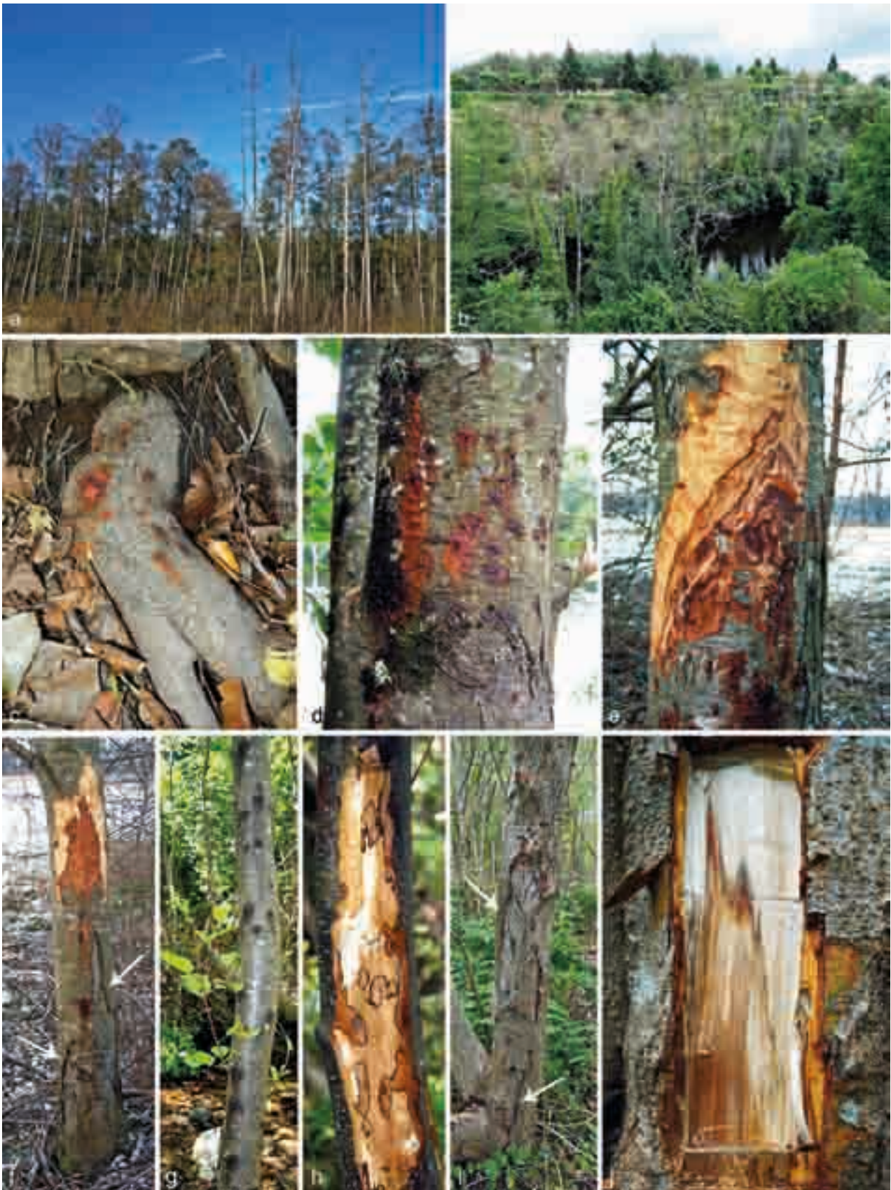
Fig. 4 Symptoms of Phytophthora root and collar rot of Alnus spp. in Europe. a. Severe dieback and mortality of a mature A. glutinosa stand caused by P. ×alni in a seasonally flooded swamp forest in Bavaria, Germany; b. extensive dieback and mortality caused by P. ×alni in a riparian stand of A. glutinosa at Rio Alva in Portugal; c. bleeding bark lesion caused by P. ×alni on a surface root of mature riparian A. glutinosa in Portugal; d. bleeding aerial bark lesion on a riparian A. glutinosa at Rio Miño in Galicia, Spain, caused by simultaneous infections of P. ×alni and P. ×multiformis in 2 m stem height during an extreme spring flood; e, f. collar rot lesions caused by P. ×alni on A. glutinosa (e) and A. incana (f) planted on a non-flooded site in Bavaria, Germany, with rusty and tarry spots on the outer bark and flame-shaped, orange-brown necrotic lesions of the inner bark; inactive older lesion areas from the previous year are sunken and surrounded by callusing tissues (arrows); g. black exudates oozing from multiple collar rot lesions caused by P. ×multiformis during a severe flood on a riparian young A. glutinosa in Sardinia, Italy, reacting with the production of epicormic shoots; h. same tree as in (g) with multiple, fresh necrotic lesions of the inner bark caused by P. ×multiformis ; i. inactive sunken collar rot lesion with surrounding callusing tissues (arrows) caused by P. siskiyouensis on a young A. cordata in the UK; j. flame-shaped staining of the xylem tissue underneath an active collar rot lesion caused by P. siskiyouensis on a young A. cordata in the UK. — Photos: a–f: T. Jung; g, h: B. Scanu; i, j: A. Pérez-Sierra.
