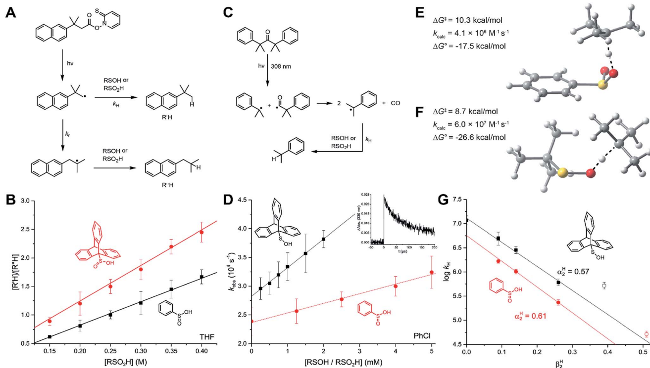
Fig. 3 (A) Photolytic generation of the 2-methyl-2-(2-naphthyl)-1-propyl radical and its use as a radical clock to obtain the rate constant for HAT from sulfenic and sulfonic acids to alkyl radicals. (B) Ratio of reduced ( R'H ) to rearranged and reduced ( R''H ) products as a function of the concentration of \text{TrptSO}_2\text{H} (red) or \text{PhSO}_2\text{H} (black) during photocleavage of the radical precursor in THF at 25 °C. (C) Photolytic generation of cumyl radicals from dicumylketone. (D) Dependence of the pseudo-first order rate on the concentration of \text{PhSO}_2\text{H} (red) and \text{TrptSOH} (black) upon photolysis of dicumylketone in \text{PhCl} at 25 °C; inset: example decay of the cumyl radical. (E and F) Calculated (CBS-QB3) transition state structures and associated free energy barriers, estimated rate constants and reaction free energies for HAT between a model alkyl radical ( t\text{-Bu}^\bullet ) and either \text{PhSO}_2\text{H} or t\text{-BuSOH} (model for \text{TrptSOH} ). (G) The HAT rate constants for \text{PhSO}_2\text{H} (red) and \text{TrptSOH} (black), determined via LFP (full symbol) and radical clock (empty symbol) plotted as a function of medium \beta_2^H .
