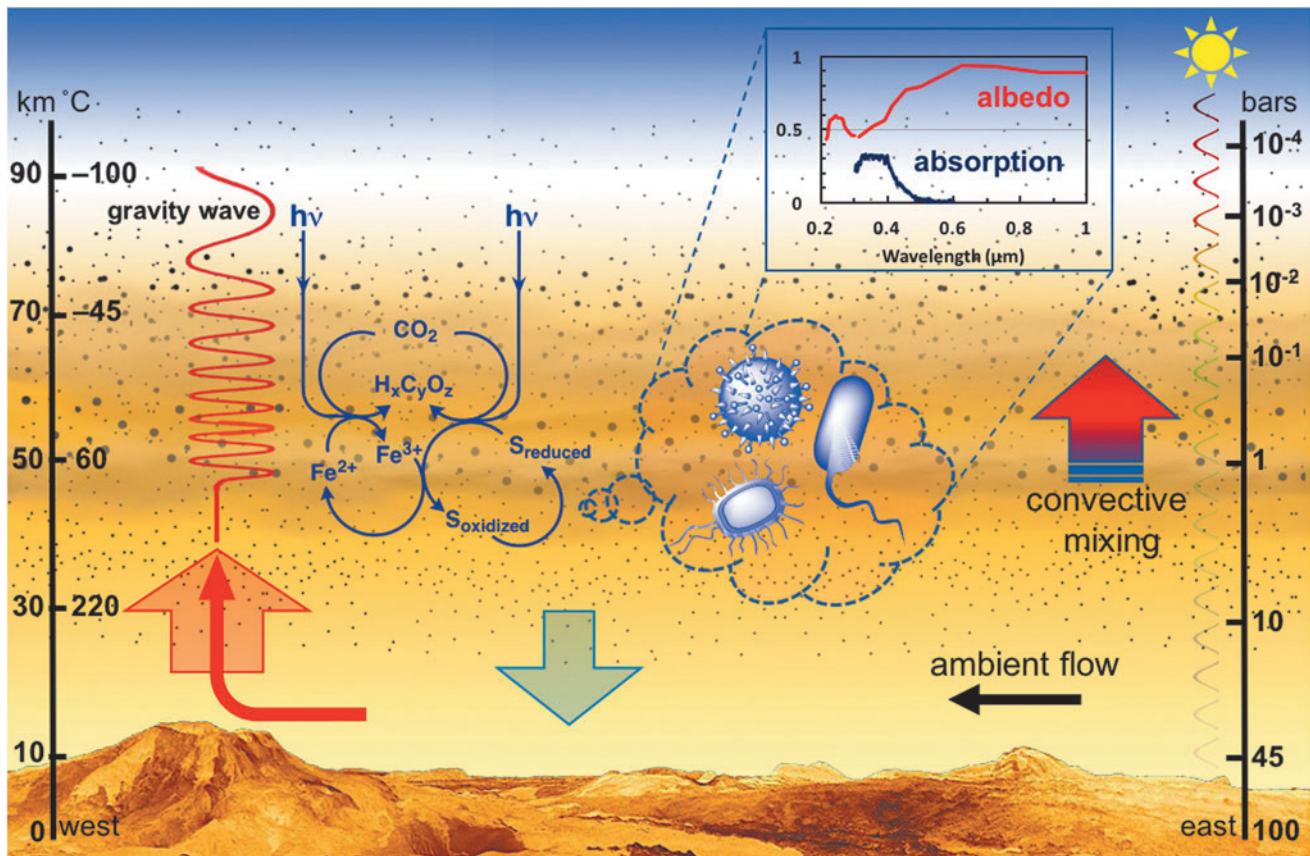
FIG. 9. A schematic representation summarizing the ideas presented in this hypothesis paper regarding the potential for microorganisms to survive in Venus' lower clouds and contribute to the observed bulk spectra. In this scheme, the approximate altitude and temperatures are shown on the left axis, the approximate pressure on the right axis, while the surface topography represents an exaggerated perspective view of Venus. The cloud layer is depicted by a yellow-tinted hazy region between an altitude of \sim 47 and 72 km, where the varying opacities and thicknesses represent differences in mass loading. The black dots within the cloud layer depict the sulfuric acid aerosols with diameters ranging from 0.2 \mu\text{m} (which are found as high as 90 km) to 2.5 \mu\text{m} and to as large as 36 \mu\text{m} (in smaller quantities) near the bottom of the cloud layer (Knollenberg and Hunten, 1980); aerosols below the cloud base have also been reported by the Venera probes. The hypothetical microbial contents of particles from the lower cloud layer are depicted in a magnified view using the dashed-line callout bubble, which shows differing possible microbial morphologies. These microorganisms may potentially survive by fixation of carbon dioxide ( \text{CO}_2 ) through the phototrophic or chemolithotrophic oxidation of iron and sulfur compounds, and by a coupled iron-sulfur metabolism (depicted by the blue reaction scheme). The cloud-based microbial communities may remain afloat through gravity waves (red wavy line), which propagate up, and are triggered by westward ambient flows over the elevated topographies; gravity waves have been detected at the cloud tops in thermal infrared in the Akatsuki data (Fukuhara et al. , 2017). Additionally, the convective activity of the lower cloud region may persist on the night side, thereby leading to opacity variations and differing thermal emissions through the cloud layer, as is observed in the near infrared in the Akatsuki and Venus Express data. Consequently, the spectra of Venus may include contributions from the cloud-based microorganisms, as is depicted by the dashed-line callout originating from the magnified view of the particles; the inset spectral plot shows the albedo of Venus compiled from differing observations (red) and the sunlight absorption estimated by a singular measurement on the dayside (at one location), as calculated from the difference between the VIRA cloud model and the MESSENGER spectra (Perez-Hoyos et al. , 2017). The absorption of sunlight may actually extend to much longer wavelengths based on muted contrasts observed by the Akatsuki orbiter (Limaye et al. , 2018), which is consistent with the albedo variation with wavelength.
