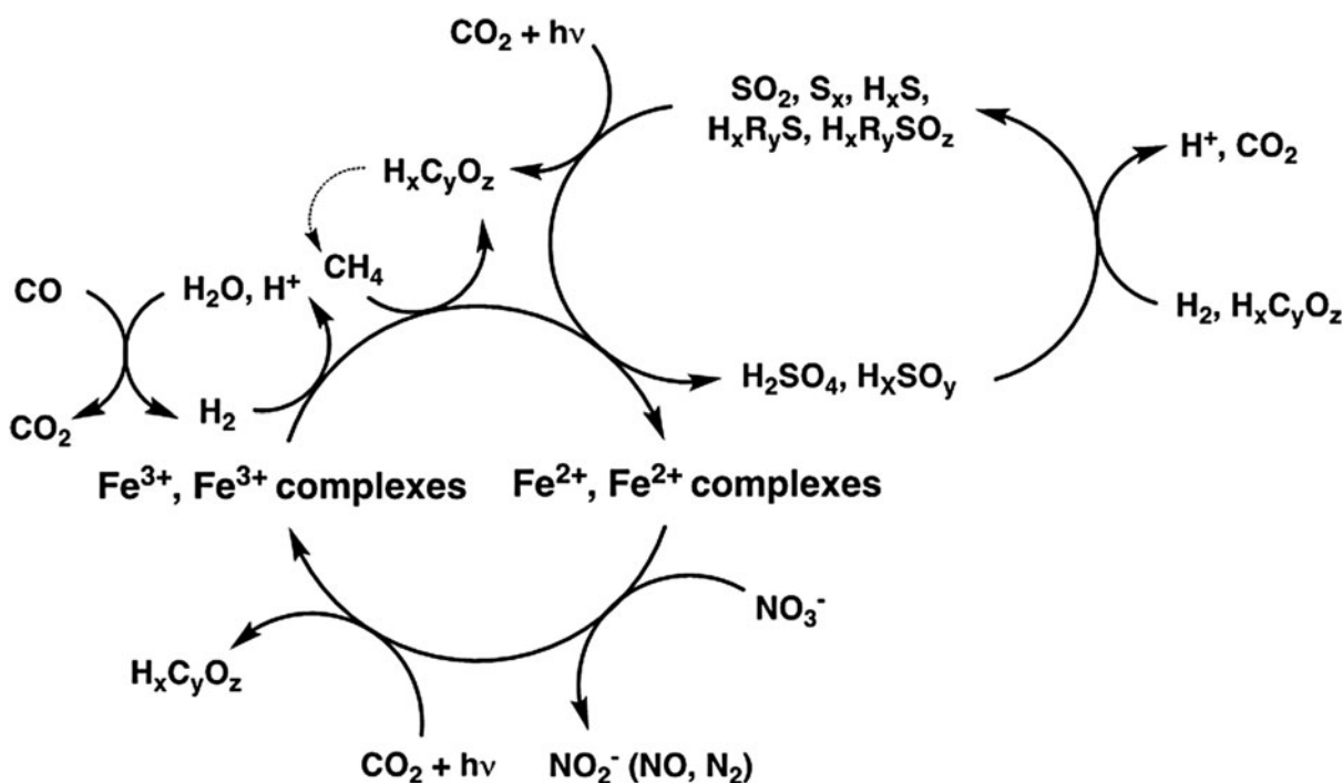
FIG. 8. Diagram of iron- and sulfur-focused metabolic redox reactions that could occur in the Venus' clouds, where \text{Fe}^{3+/2+} complexes refer to inorganic and organic ligands and dotted arrows refer to possible redox cycles.
