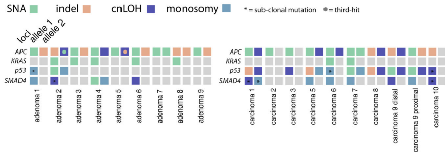
Figure 1. Mutation burdens in CRAs and CRCs
