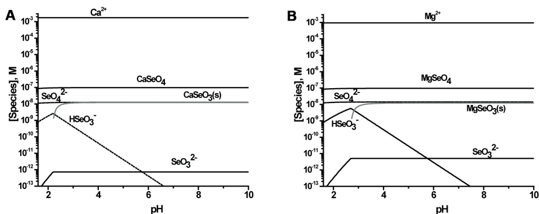
Figure 5. Speciation diagrams were calculated for LF-4 site along the Fountain Creek in the stream water with concentrations (A) of [Se(IV)] 1.2 \times 10^{-8} M, [Se(VI)] 1.1 \times 10^{-7} M and [Ca]_{\text{tot}} 1.7 \times 10^{-3} M and (B) [Se(IV)] 1.2 \times 10^{-8} M, [Se(VI)] 1.1 \times 10^{-7} M and [Mg]_{\text{tot}} 9.4 \times 10^{-4} M.
