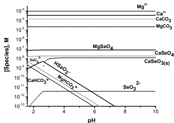
Figure 6. Speciation diagram was calculated for the LF-4 site along the Fountain Creek in the stream water with concentrations of [Se(IV)] 1.2 \times 10^{-8} M, [Se(VI)] 1.1 \times 10^{-7} M, [Ca]_{\text{tot}} 1.7 \times 10^{-3} M and [Mg]_{\text{tot}} 9.4 \times 10^{-4} M.
