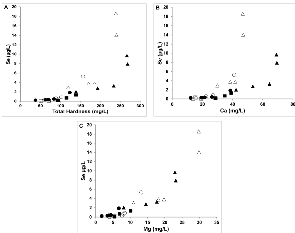
Figure 2. Total Se level ([Se]/µg/L) vs Total Hardness (A), Total Ca level (B) and Total Mg level (C) in the creek water (solid symbol) spring and (open symbol) fall 2007 in µg/L. UF is the Upper Fountain Creek (squares), MC Monument Creek (circles) and LF Lower Fountain Creek (triangles) [21]. Data points were measured in triplicates and details of the sampling sites were described.
