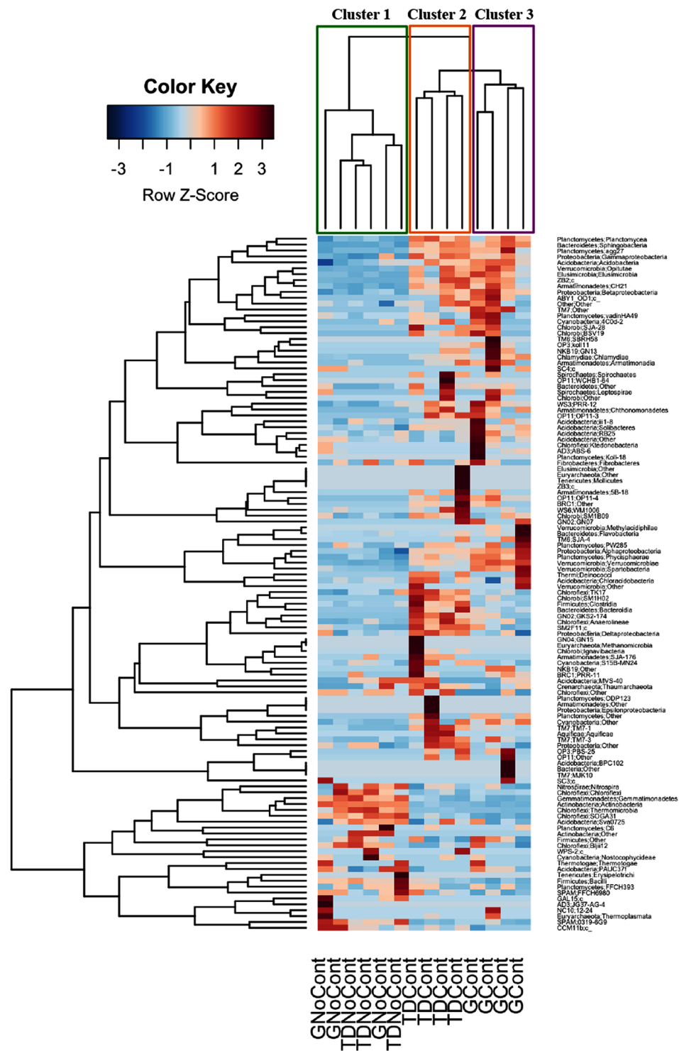
Figure 4. Heatmap representing prokaryotic taxa identified in Giugliano and Trentola Ducenta soil samples. Color scale indicates the relative abundance of each OTU within the samples. Dendrogram represents clustering patterns based on hierarchical clustering analysis on taxa and samples by Weighted Pair Group Method with Arithmetic Mean (WPGMA) method. GCont: contaminated soils at Giugliano site; GNoCont: noncontaminated soils at Giugliano site; TDCont: contaminated soils at Trentola Ducenta site; TDNoCont: noncontaminated soils at Trentola Ducenta site.
