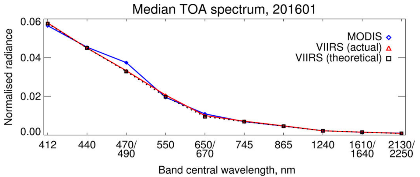
Figure 4. Median spectral observed TOA Sun-normalised radiance for MODIS (blue) and VIIRS (red) bands, and (black dashed) modelled expected VIIRS signal, after the AOD estimation and filtering steps described in Section 3.3.3. Data are from January 2016.
