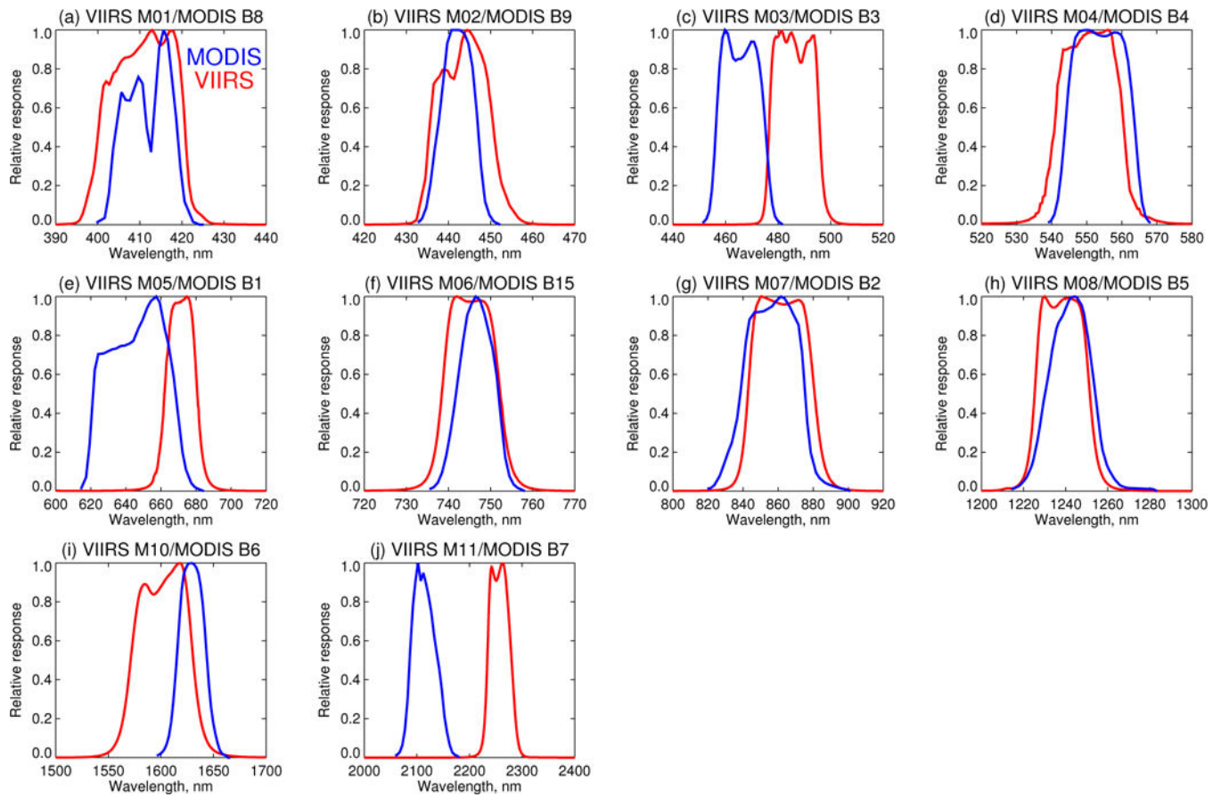
Figure 1. Relative spectral response functions for VIIRS (red) and MODIS (blue) bands used in this study (cf. Table 1).
