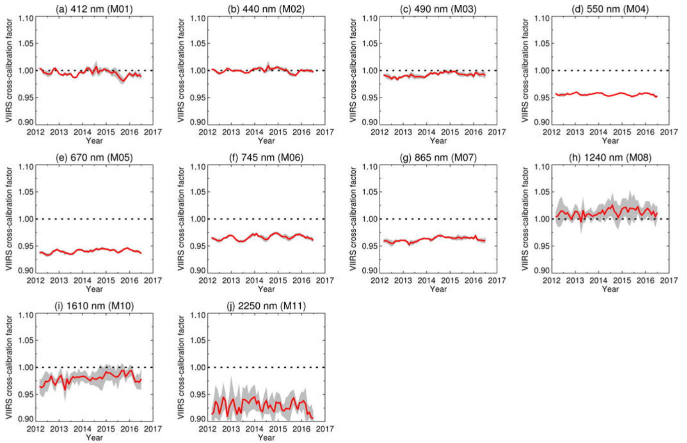
Figure 9. Time series of monthly mean VIIRS gain correction factors derived for each band (c.f. Figure 5). Red lines indicate the mean value for a month and the shaded grey area the standard deviation within a month.
