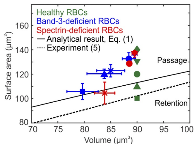
Fig. 5. Prediction of splenic IES retention for healthy RBCs (no protein deficiency) and HS RBCs. Healthy RBCs (green color symbols) with surface area of 140 (♦), 130 (▼), 120 (●), 110 (▲), and 100 μm 2 (■) and a fixed volume of 90 μm 3 are examined, respectively. The surface area and volume of HS RBCs after their passage through IES are plotted. Blue color symbols denote the band-3-deficient RBCs with vertical connectivities of 80% (▼), 60% (●), 40% (×), 20% (▲), and 0% (■). Red color symbols denote the spectrin-deficient RBCs with spectrin density of 80% (▼), 60% (●), and 40% (×). The error bars are computed based on pressure gradient values of 5, 8, 10, 15, and 20 Pa \mu\text{m}^{-1} . The black solid and dashed lines highlight the RBC retention threshold predicted by an analytical model given by Eq. 1 (19, 26) and the threshold reported by ex vivo experiment (5), respectively. RBCs with surface area and volume above these thresholds are able to cross IES; otherwise, RBCs are retained by IES.
