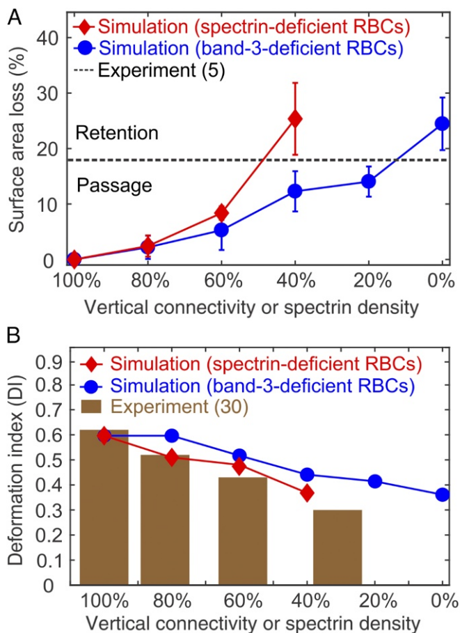
Fig. 4. (A) Fractional surface area loss of HS RBCs after passage through IES. For the band-3-deficient RBCs, the surface area loss is increased with the decreased vertical connectivity. For the spectrin-deficient RBCs, the surface area loss is increased with the decreased spectrin density. The error bars are computed based on pressure gradient values of 5, 8, 10, 15, and 20 Pa \mu\text{m}^{-1} . The black dashed line highlights the critical fraction of surface area loss that determines the retention of RBCs reported by ex vivo experiment (5). (B) DI of the band-3-deficient and the spectrin-deficient RBCs at different levels of HS-related protein deficiency. The brown bar graph shows DI of spectrin-deficient RBCs measured by osmotic gradient ektacytometry at a fixed osmolality of 300 mOsmol/kg (30).
