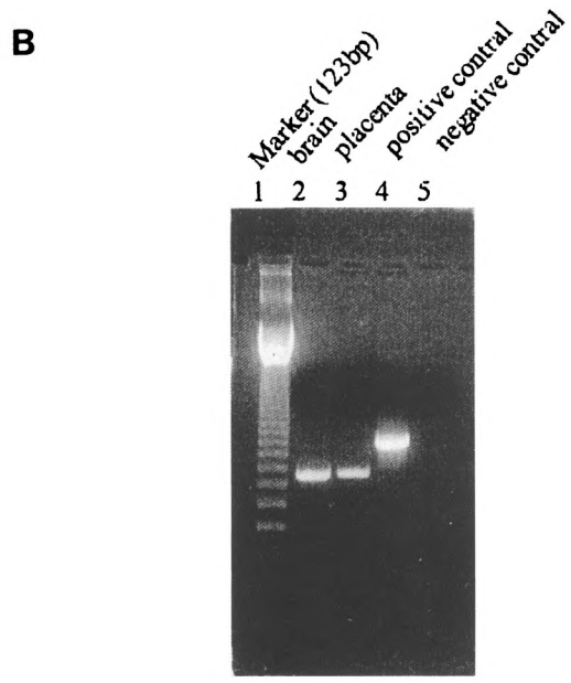
FIG. 4. Northern analysis of ML-1 mRNA expression in normal human tissue. The blot (MTC TM ) used here was purchased from Clontech, Inc. Each lane of the blot contains approximately 2 µg of purified poly(A) + mRNA from normal human brain and placenta. The probes were labeled by PCR using a pair of gene-specific primers and probed at 1 \times 10^6 cpm/ml. Arrows indicate the location of the ML-1 targets and asterisk (*) indicates the presence of HPRT that was used as a positive control (A). The data presented here were supported and confirmed by RT-PCR reaction and analysis of the products using G3PDH as a positive control (B). The primer mix was supplied by Clontech, Inc.
