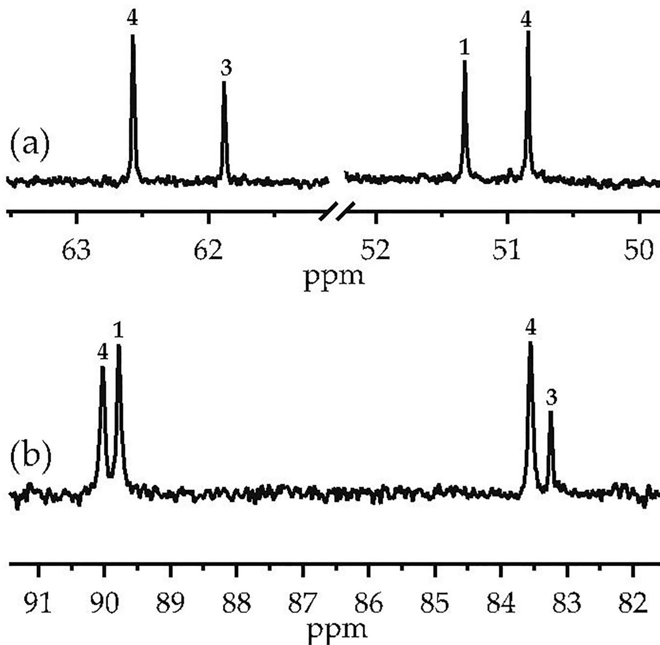
Figure 1. NMR spectra of a ~1:1 mixture (0.10 M total titer) of sodium diisopropylamide (NaDA; 1 ) and sodium dicyclohexylamide (NaDCA; 3 ) in neat dimethylethylamine (DMEA) affording heterodimer 4 . (a) ^{13}\text{C} NMR spectrum recorded at -80^\circ\text{C} ; (b) ^{15}\text{N} NMR spectrum using ^{15}\text{N} NaDA and ^{15}\text{N} NaDCA recorded at -100^\circ\text{C} .
