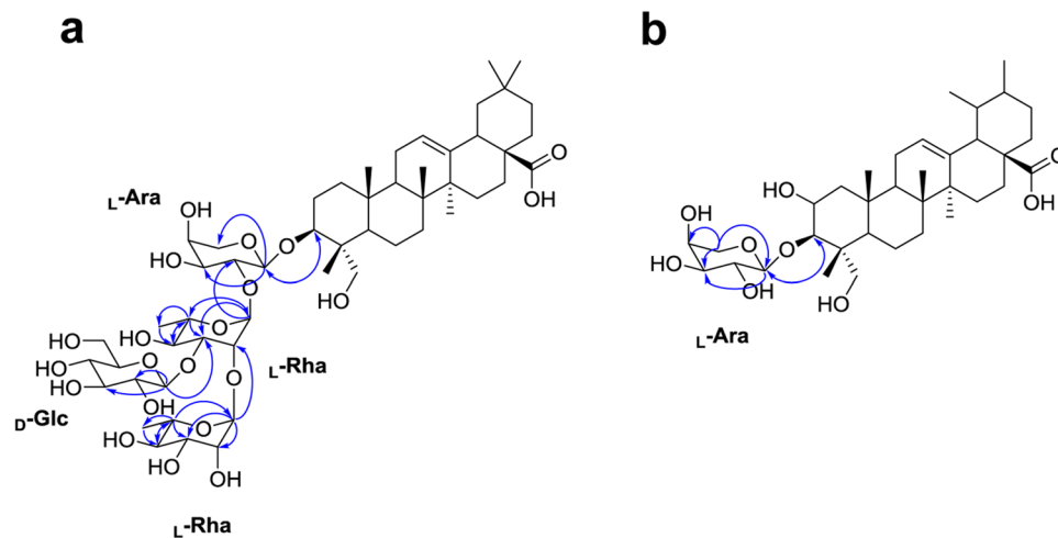
Figure 2. Key correlations to determine the positions of the glycosidic linkages in the oligosaccharide moiety of TPG1 (a) and TPG5 (b) in the HMBC spectra. The arrow lines represent the ^2J(C,H) or ^3J(C,H) correlation across the glycosidic linkages.
