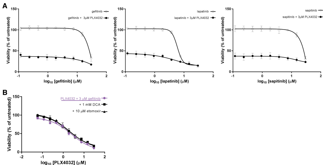
FIG. 6. Assessment of WiDr CRC cell growth by combination treatments of BRAF i and ERBB or metabolic inhibitors. A , Comparison of mono- and double therapy on WiDr CRC cells growth. All three graphs show inhibition of either EGFR, EGFR/ERBB2 or EGFR/ERBB2/ERBB3 is ineffective as a monotherapy. Moreover, concomitant inhibition of ERBB2 and ERBB3 does not provide further benefit to the synergistic effect of BRAF(V600E) and EGFR inhibitors. B , WiDr cell confluence is measured comparing double and triple treatments. The addition of etomoxir or DCA as third metabolic inhibitors after 96 h does not show additional benefit to the BRAF i +EGFR i treatment.
