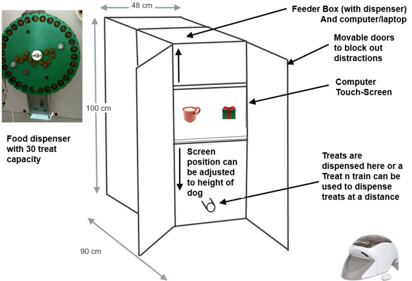
Figure 1. Schematic diagram of the touchscreen apparatus, including: Feeder box (containing food dispenser and computer/laptop), movable doors to block out distractions, and adjustable computer touchscreen. Treats are dispensed through a tube from the feeder box, or a feeding device such as the Treat & Train can be used to dispense treats at a distance. Top left: Photograph of the food dispenser used in the studies. Bottom right: Treat & Train automatic food dispenser with remote control.
