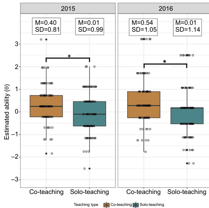
Figure 2 Comparison of equated and scaled exam score by teaching type. Notes: *statistical significance, p -value <0.05 .
