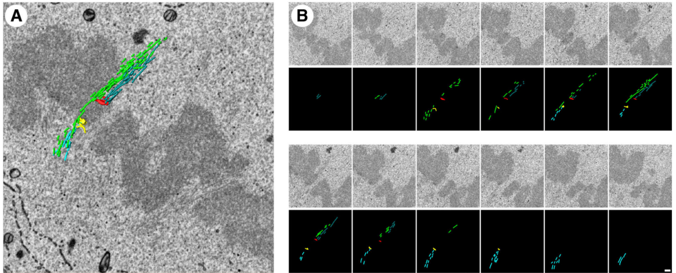
Fig. 8. Example of a putative bridging fiber.
