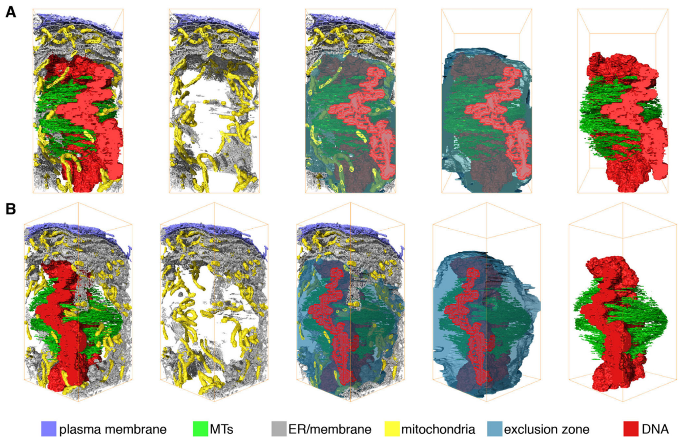
Fig. 7. The spindle exists in an ‘exclusion zone’.
