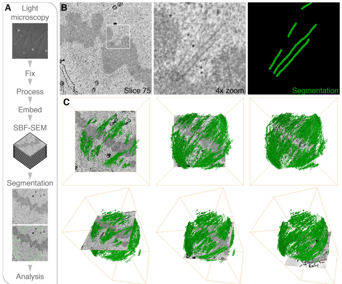
Fig. 1. SBF-SEM of mitotic spindles.
