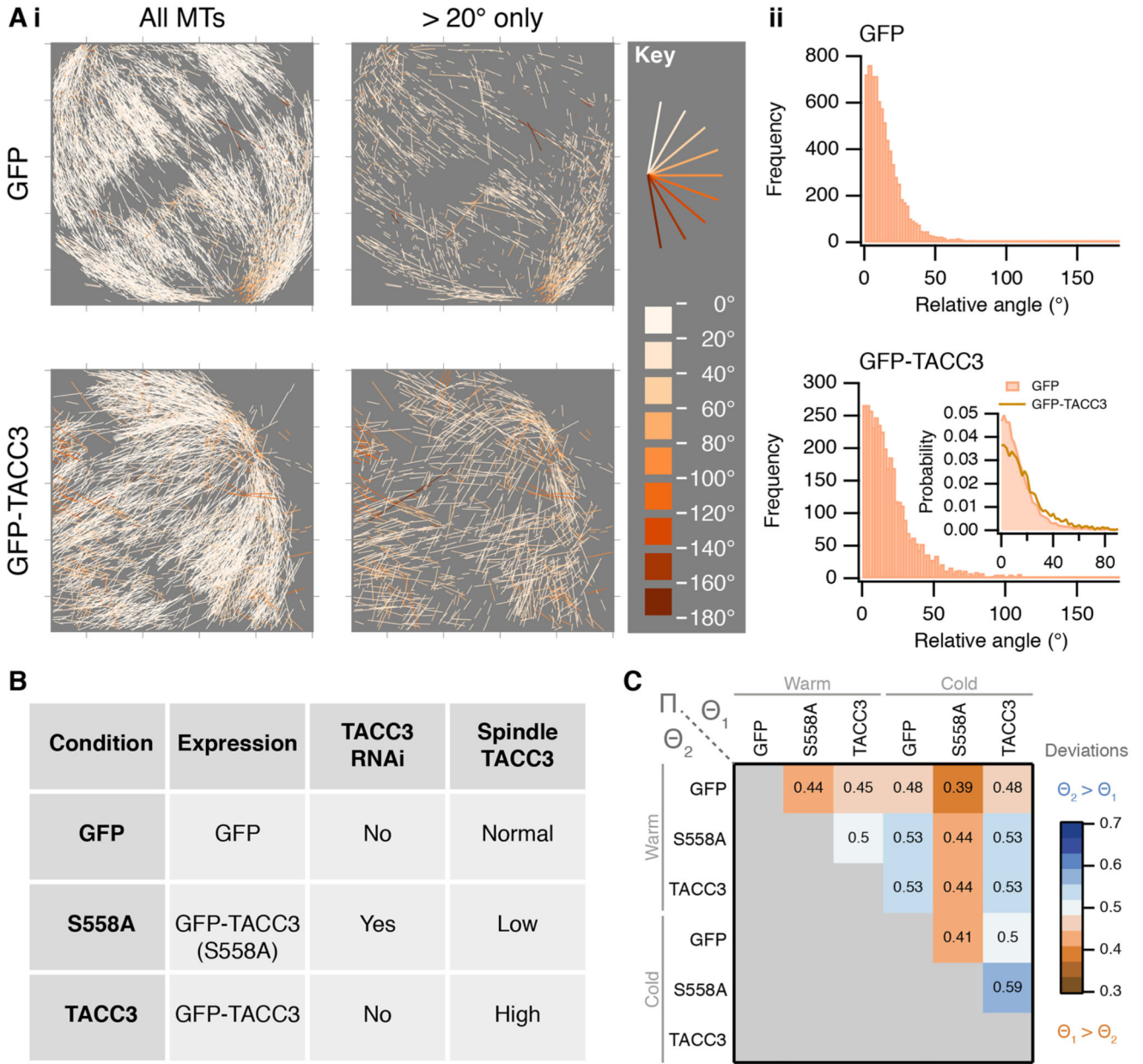
Fig. 5. A statistic for microtubule order in mitotic spindles.
