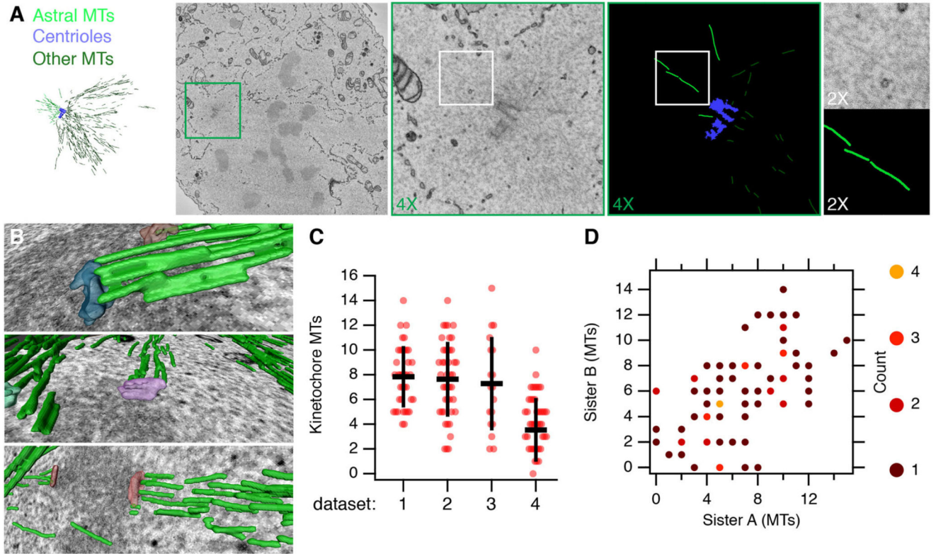
Fig. 2. Single MTs can be resolved in subsections of SBF-SEM image stacks.
