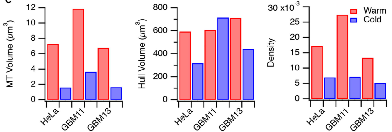
Fig. 3. Volume calculations for mitotic spindles.
