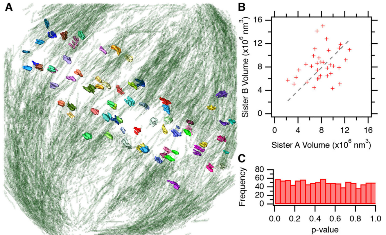
Fig. 6. Volumetric analysis of kinetochores.
