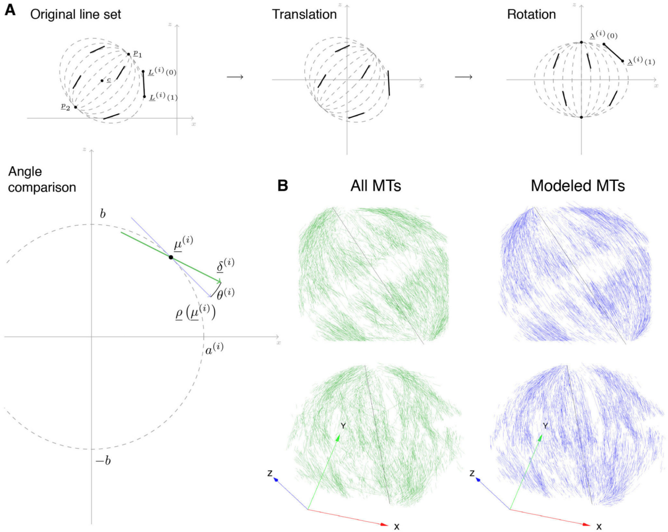
Fig. 4. Using a simple geometric model to obtain idealized mitotic spindles from measurement data.
