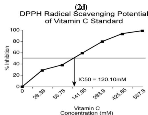
Fig. 2. Naringenin prevented the production of reactive nitrogen species, inhibited synthetic DPPH radical, and inhibited the peroxidation of unsaturated lipids present in mice brain homogenates. The ability of naringenin to inhibit RNS production was analyzed by the Griess Ilosvays reaction using sodium nitroprusside. The IC50 of naringenin was 185.6 µM (2a). The nitric acid radical-scavenging potential of vitamin C standard showed an IC50 of 130.42 µM (2b). The ability of naringenin to scavenge synthetic DPPH radical was tested according to Burits and Bucar (2000). The IC50 of naringenin was 264.44 mM (2c). The DPPH radical-scavenging activity of the vitamin C standard showed an IC50 of 120.10 mM (2d). Naringenin inhibited the peroxidation of unsaturated lipids present in mice brain homogenates. The percentage inhibition of lipid peroxidation increased with naringenin concentration (2e).
