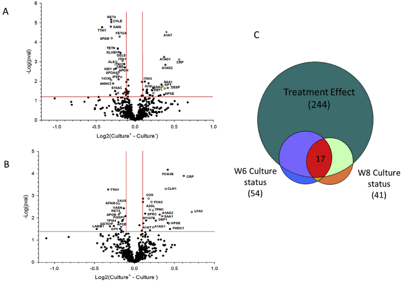
Fig. 4. Plots and diagram of proteins significantly altered based upon culture status at week 6 and week 8 treatment. Volcano plot showing log 2 values calculated from the difference of fold change from baseline to week 8 for culture positive (culture+) patients compared to culture negative (culture-) patients at (a) Week 6 culture status and B) Week 8 culture status based upon a linear mixed model. Proteins labeled are those most significant and found in common across both week 6 and week 8 results. C) Venn diagram representing overlap between the 244 treatment serum proteins and discriminatory proteins for week 6 and week 8 culture status stratification.
