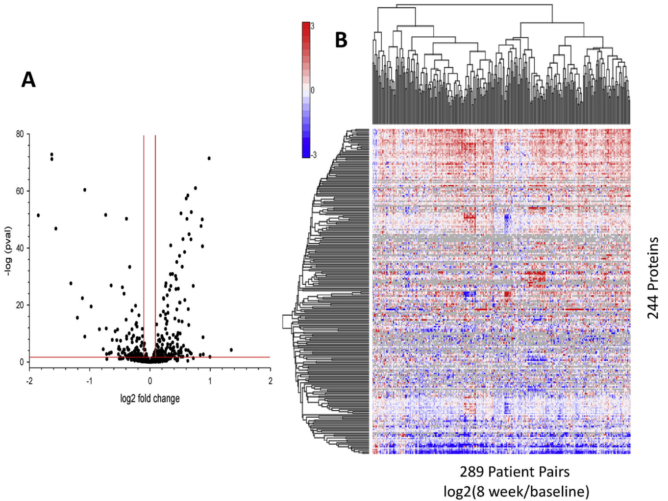
Fig. 2. Visual representation of the serum proteins differential abundant due to 8 weeks of antibiotic treatment. A) Volcano plot of all proteins analyzed via linear mixed model to determine differential abundance due to antibiotic treatment at 8 weeks. Red lines correspond to thresholds of acceptance ( pval < 0.05 and > \pm 0.1 \log_2 fold change). B) Heat map of 244 proteins representing quantitative changes in protein abundances between baseline and 8 weeks from 289 patients. Red magnitude representing increase in abundance with treatment, blue magnitude representing reduced serum abundance upon treatment. (For interpretation of the references to colour in this figure legend, the reader is referred to the Web version of this article.)
