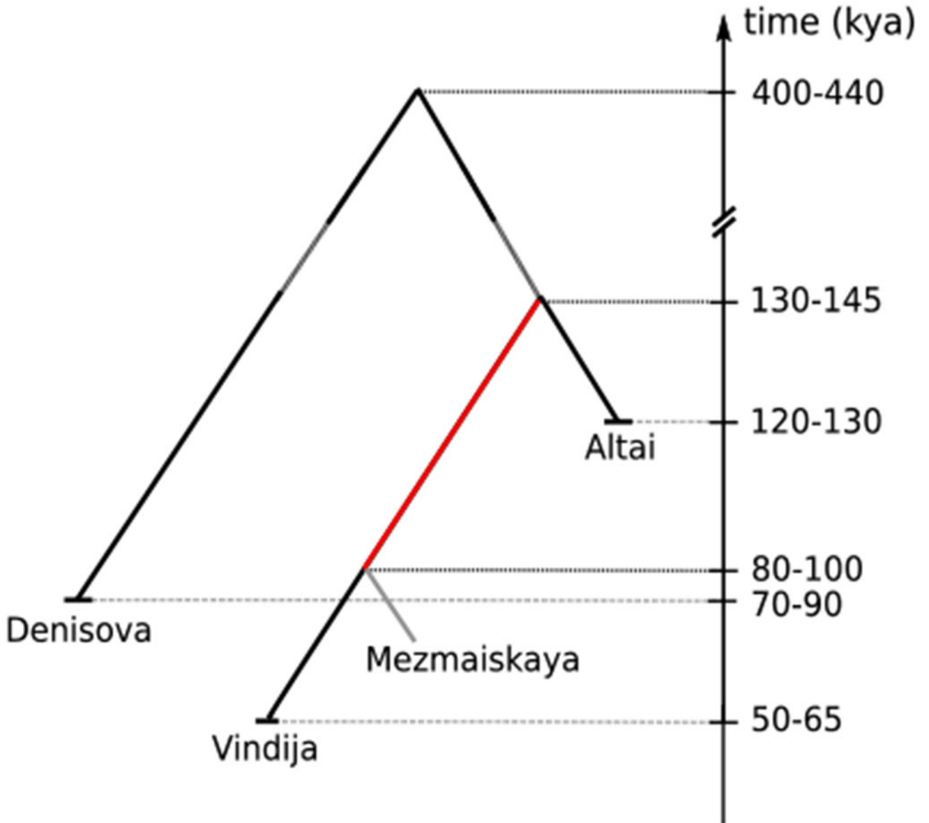
Fig. 2. Approximate ages of specimens and population split times.
