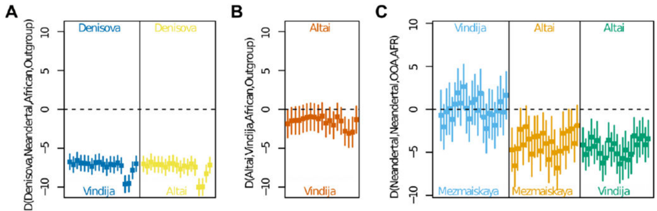
Fig. 3. Allele sharing between archaic and modern humans.
