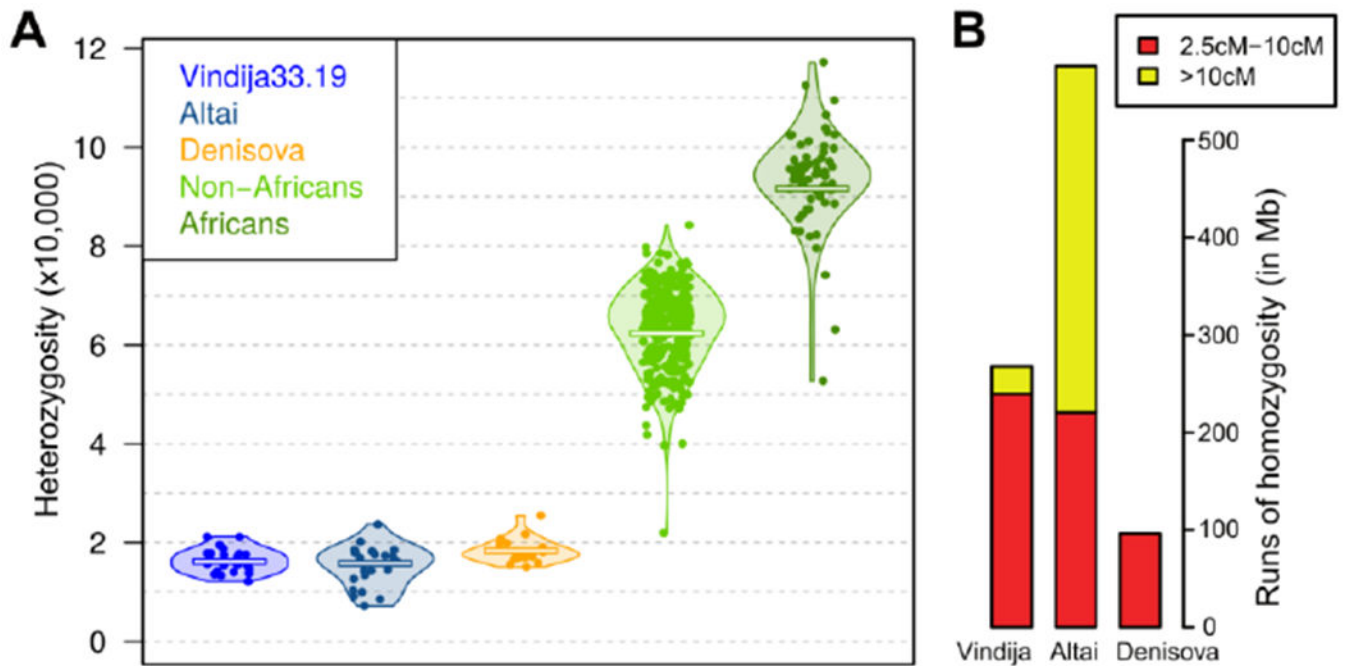
Fig. 1. Heterozygosity and inbreeding in the Vindija Neandertal.
