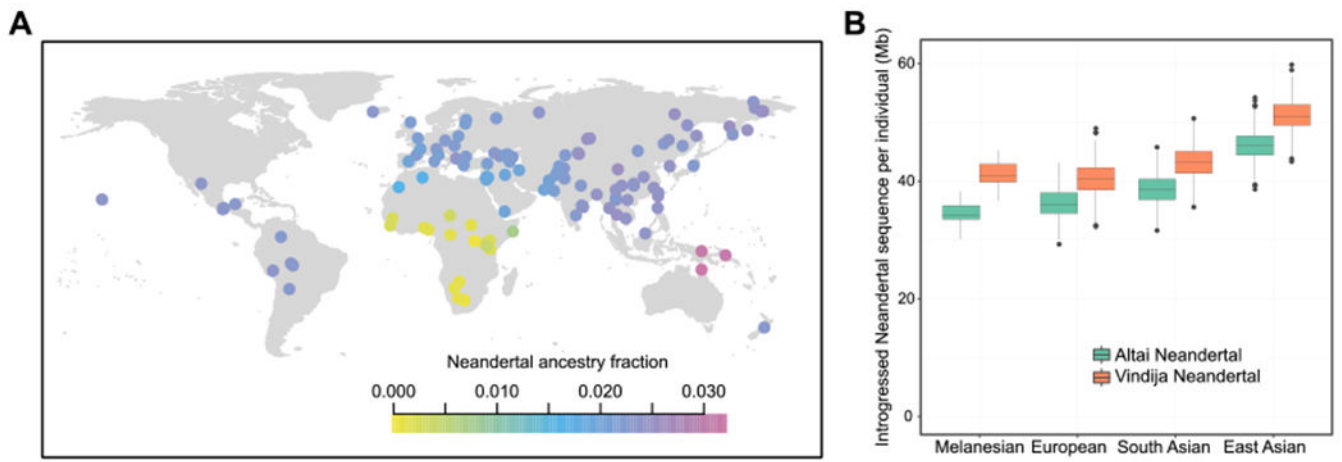
Fig. 4. Estimates of fraction of Neandertal DNA for present-day populations.
