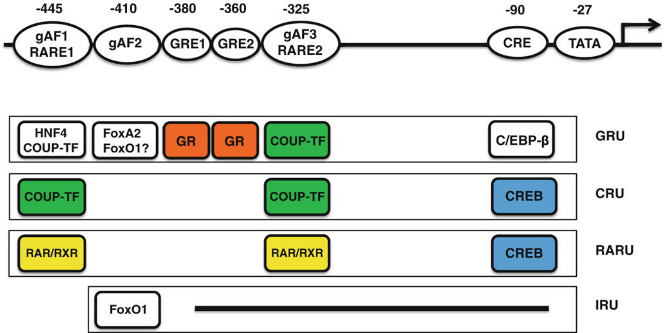
Fig. 5.3. Hormone response units in the PEPCK gene. Binding sites for various regulatory and transcription factors are shown in the top row , with the number indicating the center nucleotide position of each element with respect to the transcription start site. Four hormone-specific response units are drawn: proximal glucocorticoid response unit (GRU), cyclic AMP response unit (CRU), retinoic acid response unit (RARU), and insulin response unit (IRU). In the absence of the other hormones, the components of each response unit are depicted. These units interact functionally, cooperating or competing, to comprise the PEPCK promoter. Except for gAF2, DNA elements involved in IRU are not yet identified
