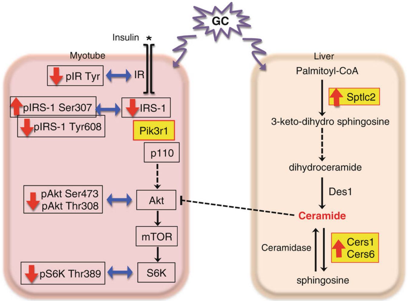
Fig. 5.4. Models of glucocorticoid-regulated insulin action. Mechanisms of glucocorticoid-induced insulin resistance are depicted. In myotubes, glucocorticoids (GC) decrease the tyrosine phosphorylation of insulin receptor (IR) and the expression of IRS1. They increase the serine 307 phosphorylation while decrease the tyrosine 608 phosphorylation of IRS1. GC also increase the expression of Pik3r1, which results in decreased activity of Akt and p70 S6 kinase (S6K). In the liver, GC increase the gene expression of enzymes involved in ceramide synthesis, including Sptlc2, Cers1 and Cers6, which results in increased levels of ceramides. These ceramides then interfere with insulin signaling. The GC-regulated genes are shown in yellow
