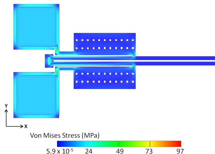
Figure 16. Von Mises stresses developed within the polysilicon microgripper structure at a potential of 3 V.
