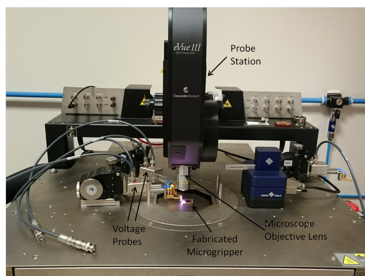
Figure 10. The fabricated microgripper enclosed in an integrated circuit (IC) package and mounted on the platform of the vibration isolation Cascade Microtech probe station with voltage probes to actuate the microgripper structure.
