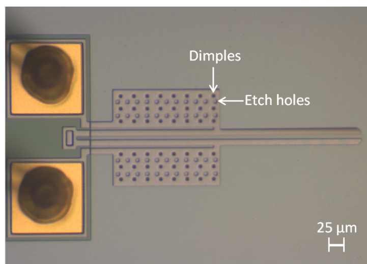
Figure 3. Optical microscope image of the fabricated polysilicon microgripper, also showing the gold wire bond interconnections on the probe pads for electrical activation of the structure.
