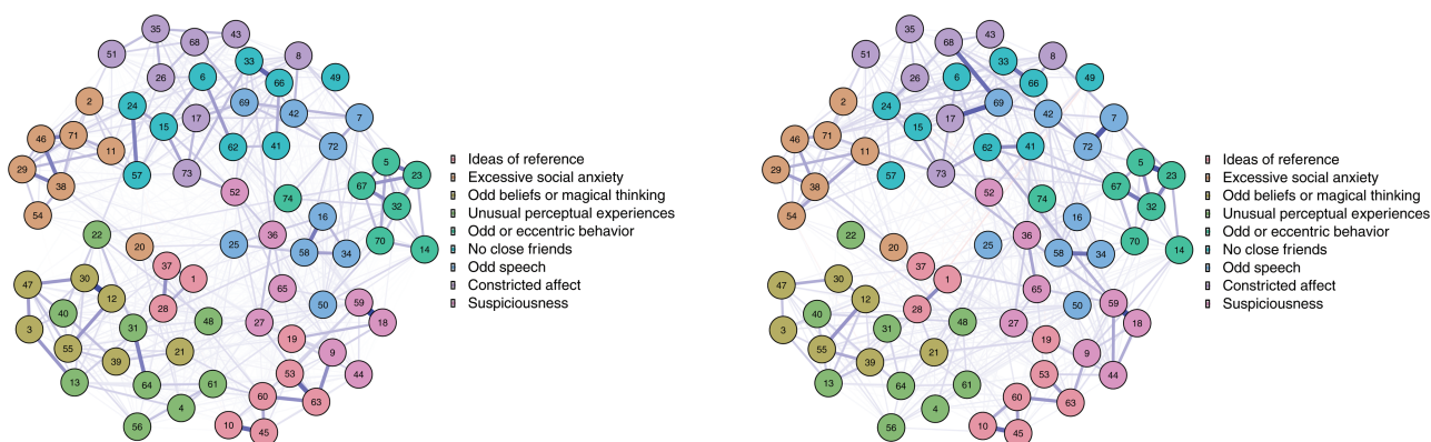
Fig. 7. Ising models of North America (left) and China (right). Blue edges are positive associations, and red edges are negative ones. Thickness and saturation of edges depict the strength of associations. The numbers refer to the SPQ items provided in supplementary material .
