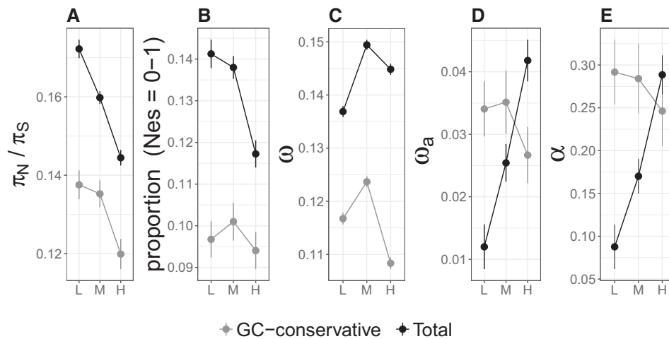
FIG. 2. Estimates of five different test statistics and 99% confidence intervals for genes in low (L), mid (M), and high (H) recombination environments for different mutation categories: GC-conservative (gray) and all sites (“Total”; black). (A) \pi_N/\pi_S , (B) proportion ( N_{eS} = 0-1 ), that is, the proportion of nonsynonymous mutations for which N_{eS} < 1 , (C) \omega , (D) \omega_a , and (E) \alpha .
