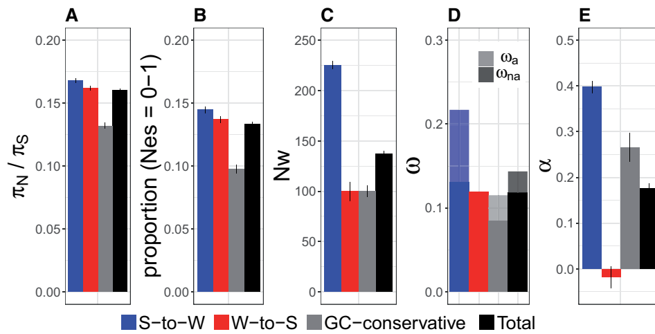
FIG. 1. Estimates of six different test statistics and 99% confidence intervals for different mutation categories: S-to-W (blue), W-to-S (red), GC-conservative (gray), and all sites (“Total”; black). (A) \pi_N/\pi_S , (B) proportion ( N_{eS} = 0-1 ), that is, the proportion of nonsynonymous mutations for which N_{eS} < 1 , (C) N_w : the weighted change in N_e relative to 100, (D) \omega , with the proportion of \omega represented by \omega_{na} and \omega_a shown in bold and light color, respectively, and (E) \alpha .
