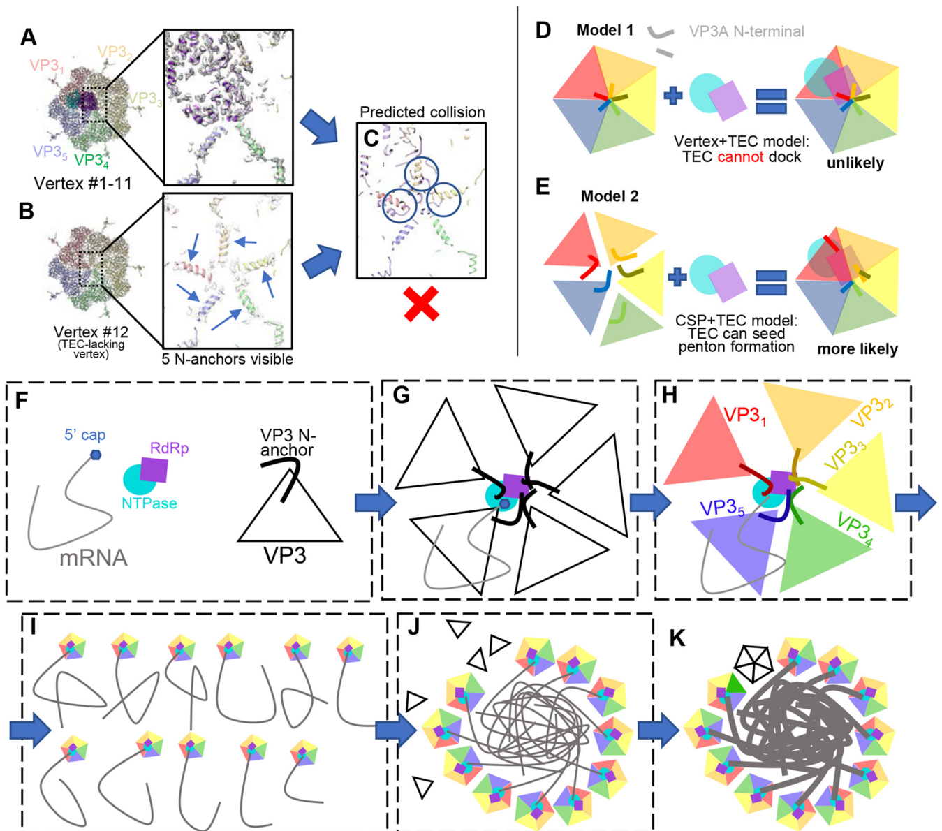
FIG 15 TEC-lacking vertex 12 and implications for the assembly mechanism. (A and B) Density map and models at vertices with (A) and without (B) a TEC. Note that in the icosahedral reconstruction, no N anchors of VP3A were visible due to averaging. (C) Direct model superposition of the TEC in panel A on five VP3As in panel B showing collision of TECs with N anchors (circled). (D and E) Two proposed models of assembly. (D) In model 1, vertices assemble first, followed by attachment of a TEC. The TECs would collide with assembled N anchors. (E) In model 2, the TEC seeds VP3A assembly, where VP3A N anchors can adapt the observed asymmetric pattern. (F to K) “Wool ball” model of virus assembly. (F) Building blocks of ARV assembly. TECs interact with mRNA and VP3, drawing the latter to their ideal positions (G), leading to properly folded N anchors around the TEC (H). The 11 genomic RNA segments, each with a vertex (I), coalesce to form a wool ball, bringing VP3s in close proximity to accelerate assembly (J). (K) Vertex 12 seals the capsid, while RdRp replicates a complementary strand from the plus-sense mRNA template in a confined environment.
