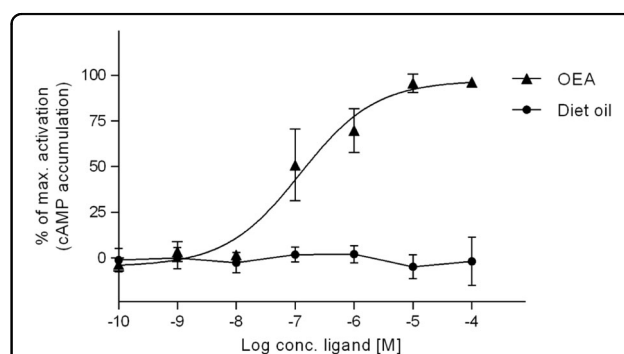
Fig. 1 In vitro. C4-Dietary-oil does not by itself activates GPR119 transiently expressed in COS-7-cells. Formation of cAMP was measured after stimulating GPR119-expressing COS-7 cells with oleoylethanolamide (OEA) and C4-dietary oil. The response is shown as percentage between full stimulation with OEA (100%) and no stimulation (0%) ( n = 3 )
