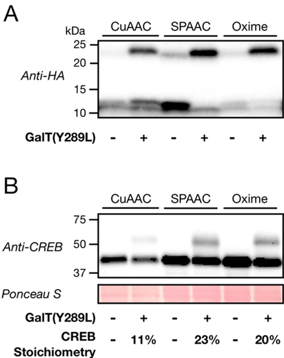
Figure 3. Comparison of mass tagging with SPAAC with CuAAC or oxime formation. (A) Cell lysates were doped with O-GlcNAcylated ubiquitin and subjected to enzymatic modification with either GalNAz (CuAAC and SPAAC) or 2-keto-galactose (Oxime) before bioorthogonal reaction with the appropriate PEG tag and visualization by Western blotting. (B) Cell lysates were subjected to the procedure described for panel A, and the endogenously O-GlcNAcylated proteins Nup62 and CREB were visualized by Western blotting. The quantification is consistent in three different biological replicates.
