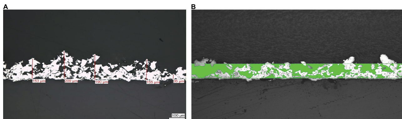
Figure 1 Exemplary sections through Ti-PEEK surface coating.
