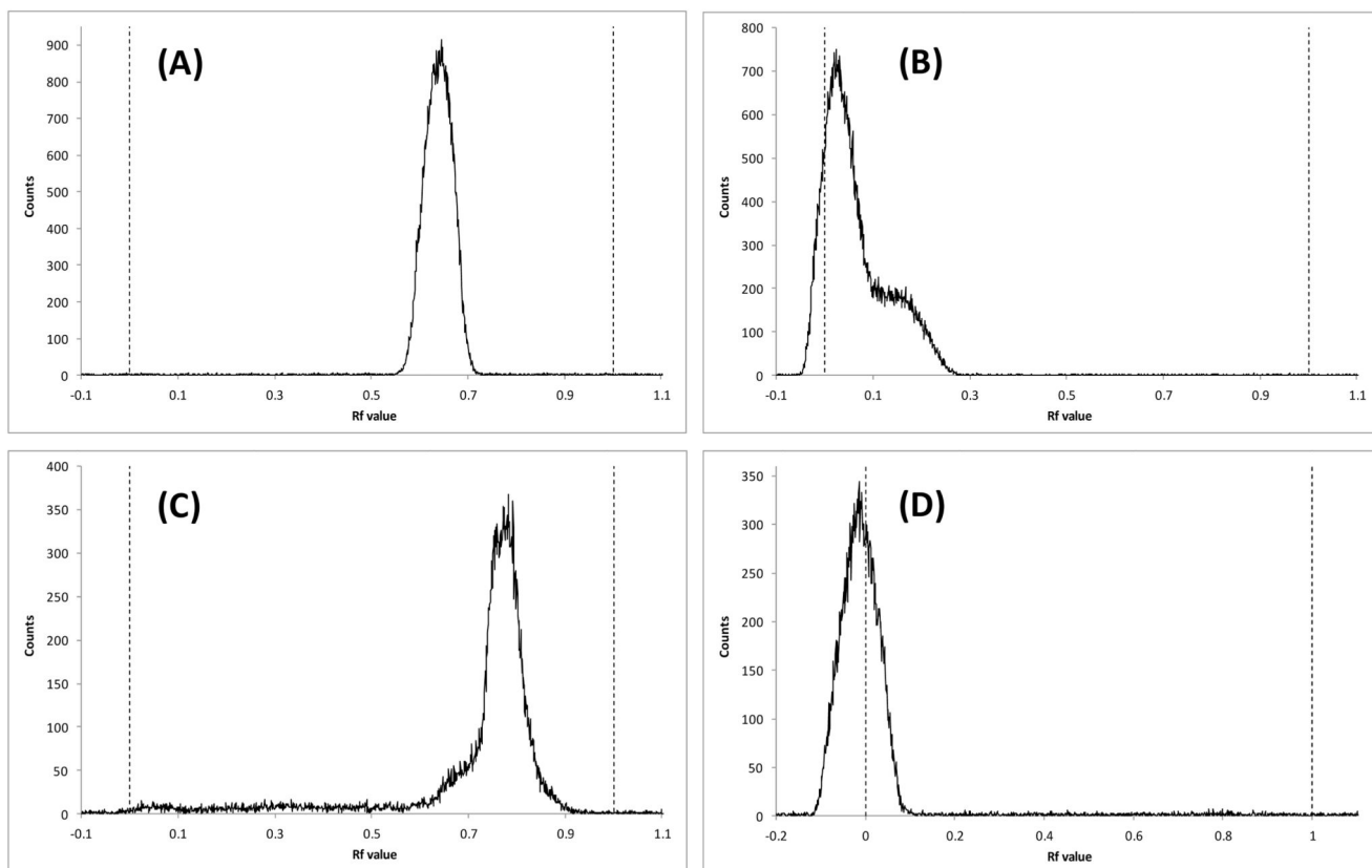
Figure 3. Radio-TLC chromatograms on silica gel coated aluminium plates of (A) ^{99m}\text{TcO}_4^- , solvent system 1; (B) ^{99m}\text{TcN}_2^+ intermediate, solvent system 1, (demonstrating the absence of pertechnetate at this stage); (C) ^{99m}\text{TcN}_2^+ intermediate, solvent system 2 and (D) ^{99m}\text{Tc-7} , solvent system 2 (demonstrating the absence of both pertechnetate and the Tc-nitride intermediate in the final product).
