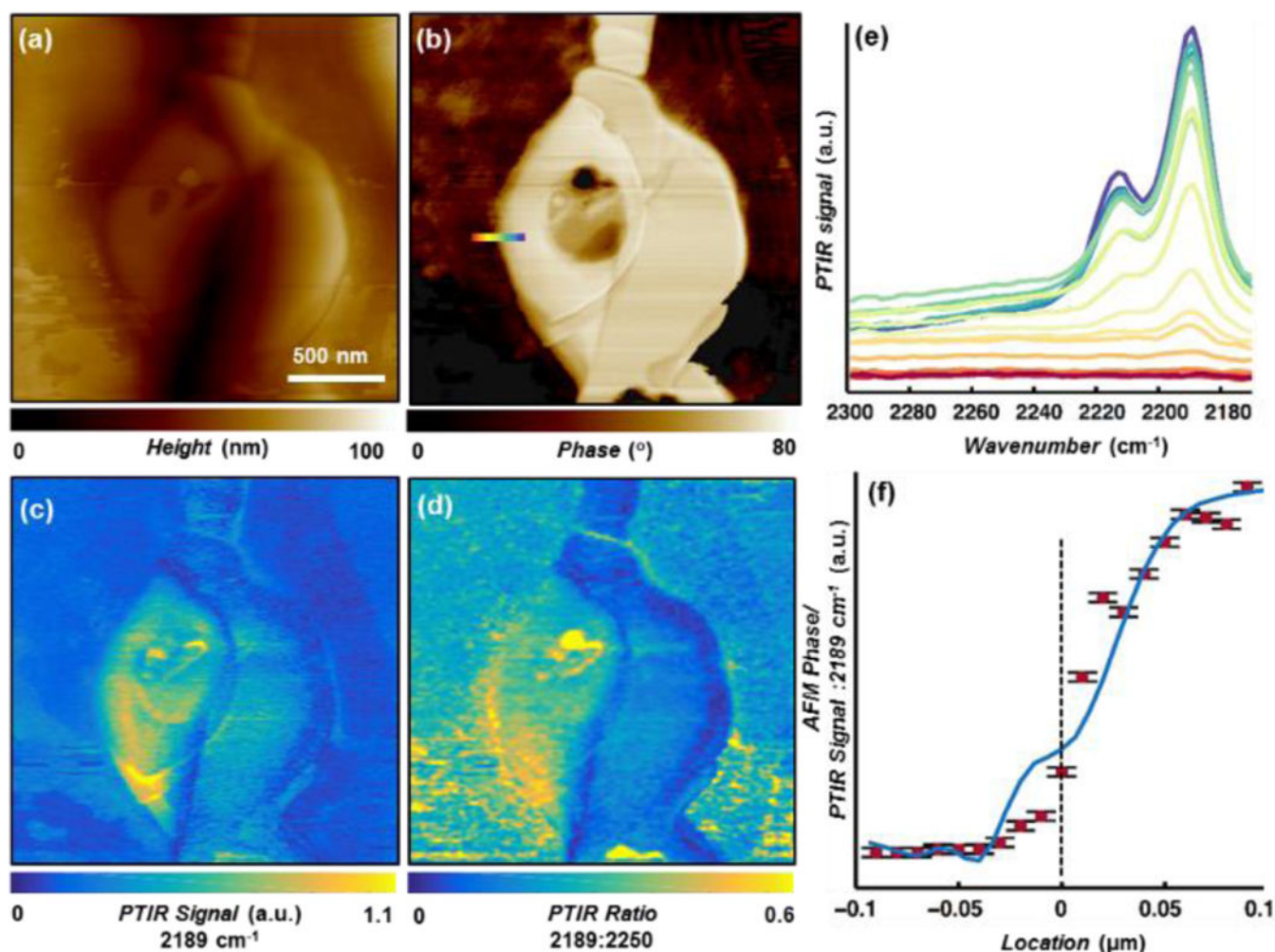
Fig. 4. (a) AFM topography map, and (b) phase map of paclitaxel loaded d-DPPC/PBD-b-PEO hybrid films. (c) PTIR absorption map (2189 cm -1 , d-DPPC symmetric CD 2 stretching), and (d) PTIR ratio image obtained by dividing the d-DPPC symmetric CD 2 stretching (2189 cm -1 ) map with respect to non-specific background absorption (2250 cm -1 ). (e) PTIR spectra obtained at the color-coded locations in panel-(b). (f) AFM phase line profile (blue) and 2189 cm -1 spectral intensity [red dots, derived from spectra in panel-(e)] across the color-coded location in panel-(b) showing an abrupt change in chemical composition. The line at “0” μm marks the edge of the lipid-rich domain, as observed in the topography image in panel-(a). Error bars represent a single standard deviation in the determination of the PTIR signal intensity.
