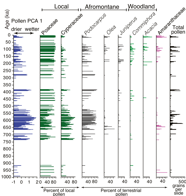
Fig. 4. Pollen stratigraphy. Selected taxa are shown. Pollen PCA 1 summarizes all pollen data and shows a long-term reduction in PCA values from ~575 ka that reflects increased aridity. Poaceae increases upward, with Cyperaceae and Podocarpus declining. Other taxa suggest increasing aridity during the last half million years.
