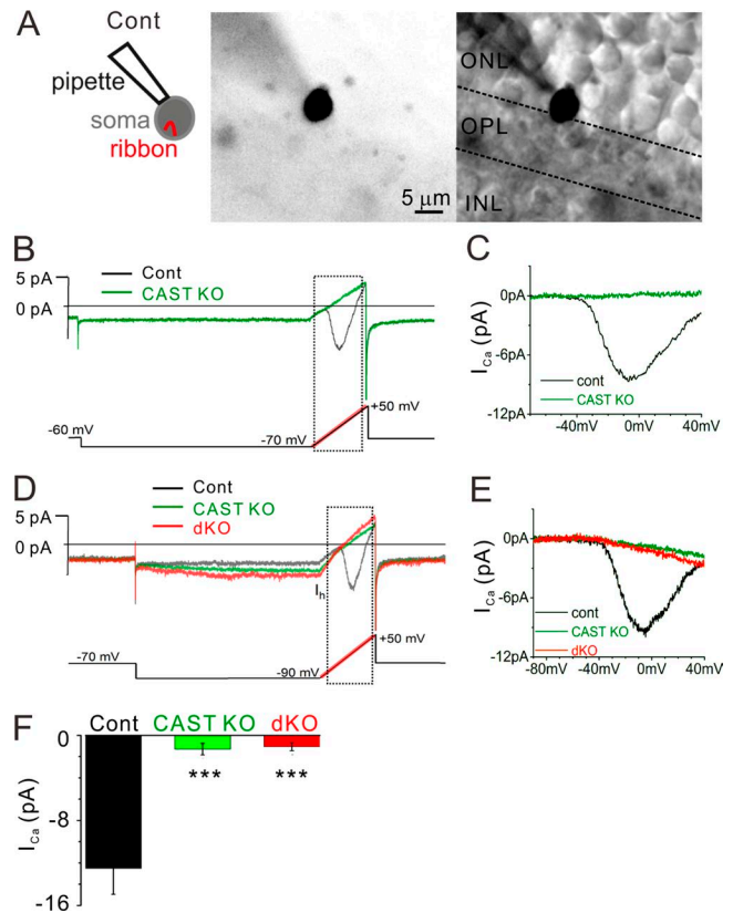
Figure 5. I_{Ca} is drastically reduced in CAST KO and dKO rod photoreceptors. (A) Representative images of a recording made from a soma located at the ONL–OPL border, where the ribbon is contained in the soma compartment. The cell is filled with an Alexa Fluor 488 via recording pipette. Bars, 5 \mu m. (B and C) Control rod current trace (black line) exhibits the current–voltage ( I – V ) behavior for rod voltage-dependent Ca_V1.4 channels (recording from the cell that is presented in A). The voltage protocol is indicated at the bottom, and the ramp portion is highlighted in red. The current response to the voltage ramp (indicated by dashed square) is leak subtracted and presented in C. In contrast to the control, the CAST KO trace (green line) lacks an inward current. (D and E) The voltage protocol further tests the excitability of the cells by stepping from -70 to -90 mV to activate a I_h . While all genotypes showed inward I_h , CAST KO and dKO mice exhibited no signs of I_{Ca} . Current traces are presented after 1 kHz low-pass filtering. (F) The average peak amplitudes including the ramps starting at -70 and -90 mV were drastically reduced in CAST KO and dKO mice. In contrast, there were no significant differences between CAST KO and dKO mice ( P < 0.7 ), mean \pm SEM. control, n = 9 cells from seven mice; CAST KO, n = 8 cells from seven mice; dKO, n = 16 cells from 11 mice; ***, P < 0.001 (two-sided Student's t test).
