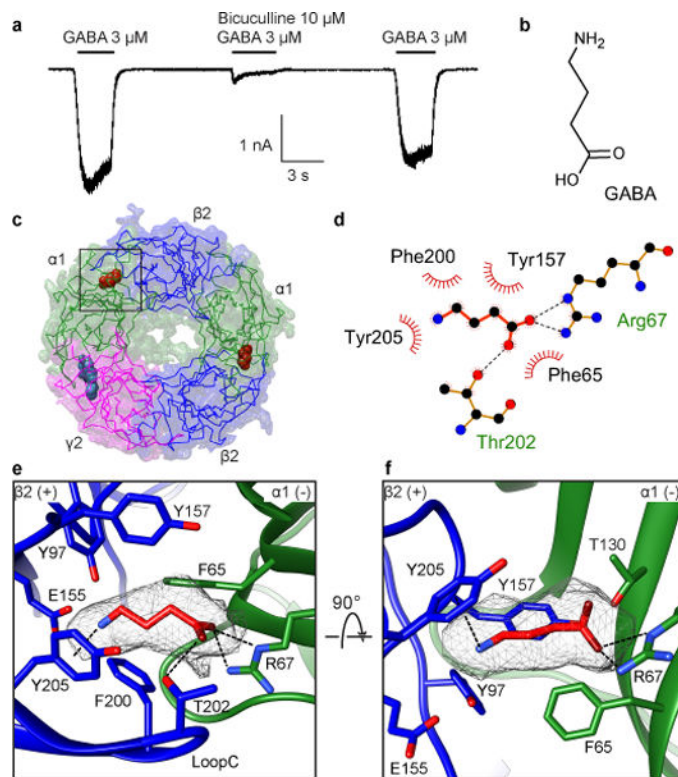
Figure 2. Neurotransmitter binding site
