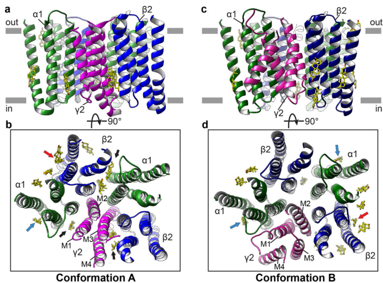
Figure 6. Conformational arrangements of transmembrane domain
